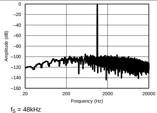
Figure 12. Dynamic Range
