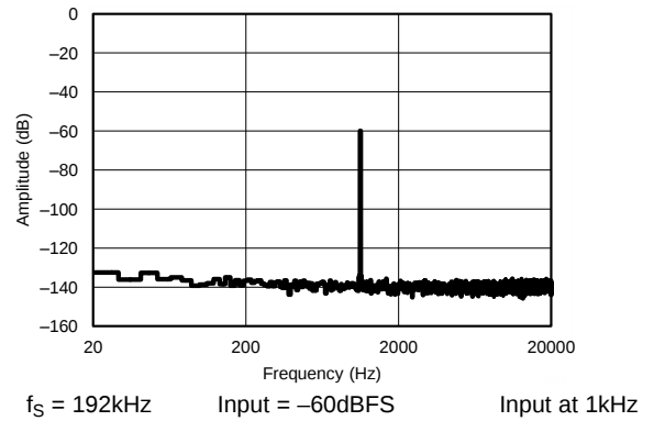
Figure 12. Dynamic Range
