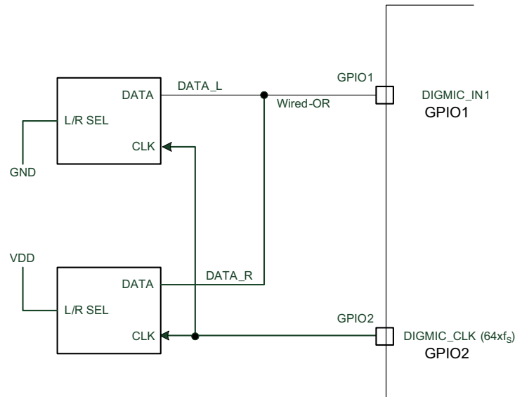
Figure 25. Digital Microphone Example Connection
