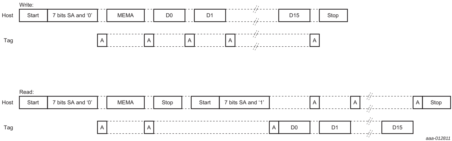
Fig 18. I 2 C READ and WRITE operation
