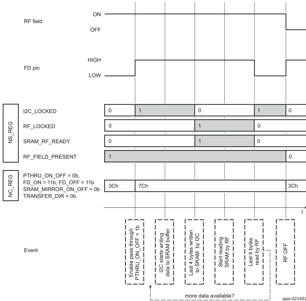
Fig 30. Illustration of the Field detection signal feature in combination with pass-through mode for data transfer from I 2 C to NFC
