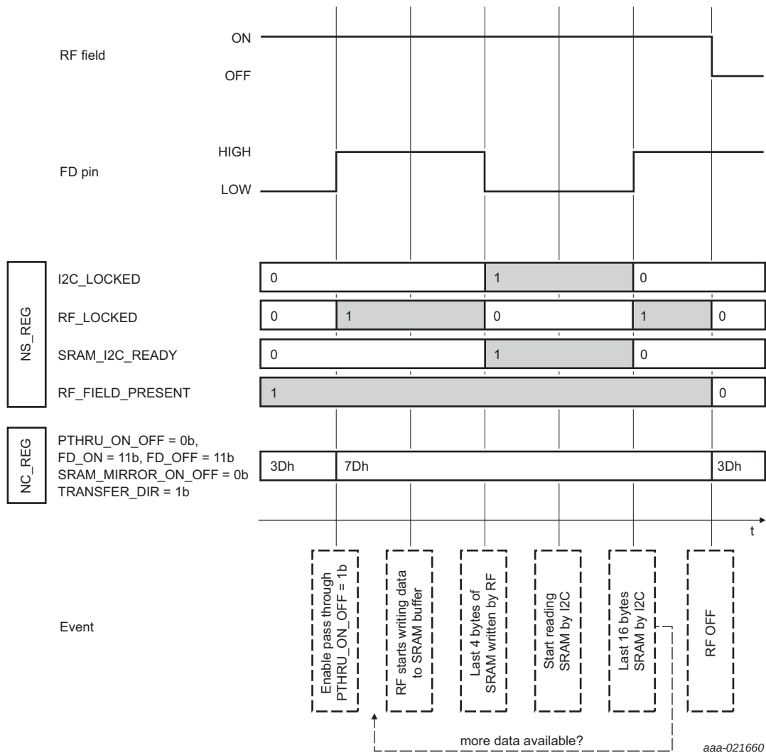
Fig 29. Illustration of the Field detection feature in combination with the pass-through mode for data transfer from NFC to I 2 C
