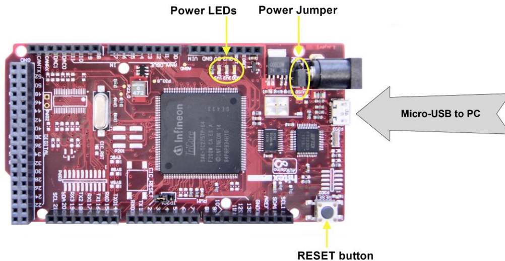
Figure 21 ShieldBuddyTC275
