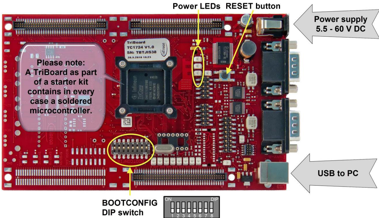
Figure 25 TC1724 - TriBoard
