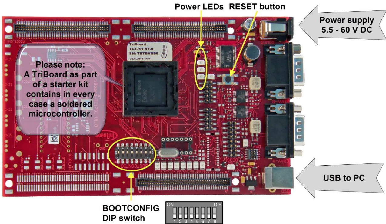
Figure 26 TC1791 - TriBoard
