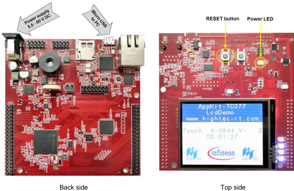
Figure 19 AURIX Application Kit TC2X5
