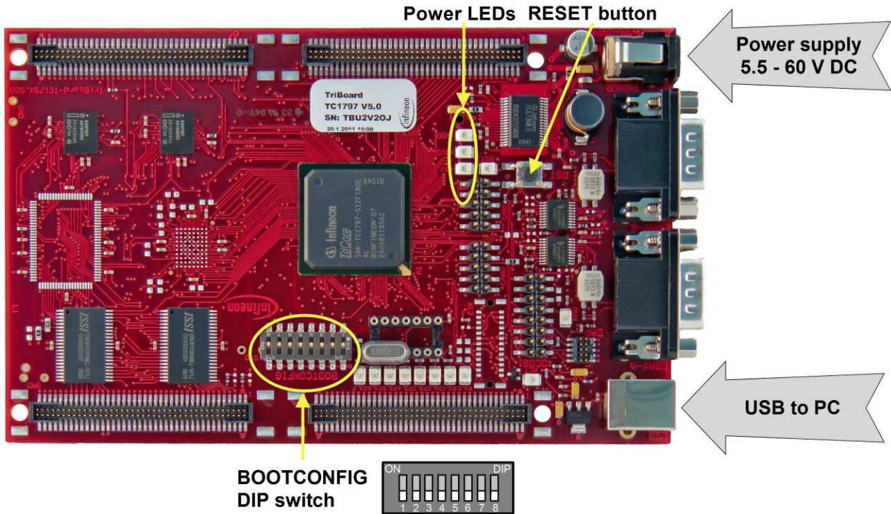
Figure 23 TC1797 - TriBoard
