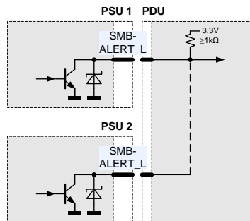
Figure 16. SMBALERT_L connection
