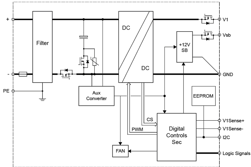
Figure 1. Block Diagram
