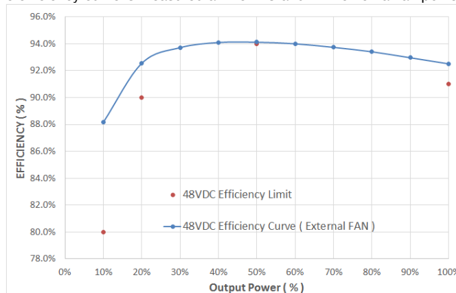
Figure 2. Efficiency Curve
