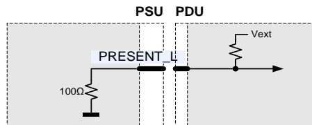
Figure 9. PRESENT_L connection
