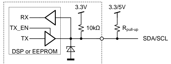
Figure 14. Physical layer of communication interface
