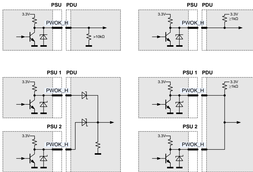
Figure 8. PWOK_H connection
