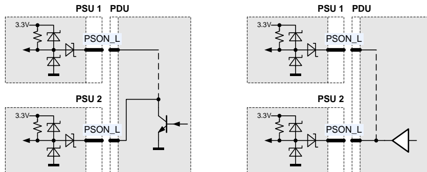
Figure 7. PSON_H connection
