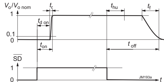
Fig. 7 Typical output response to the SD-signal. If option M is not fitted, t_{hu} = 0\ ms .
