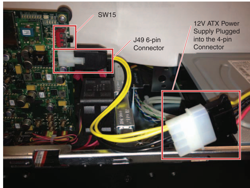
Figure 13: Power Supply Connection
