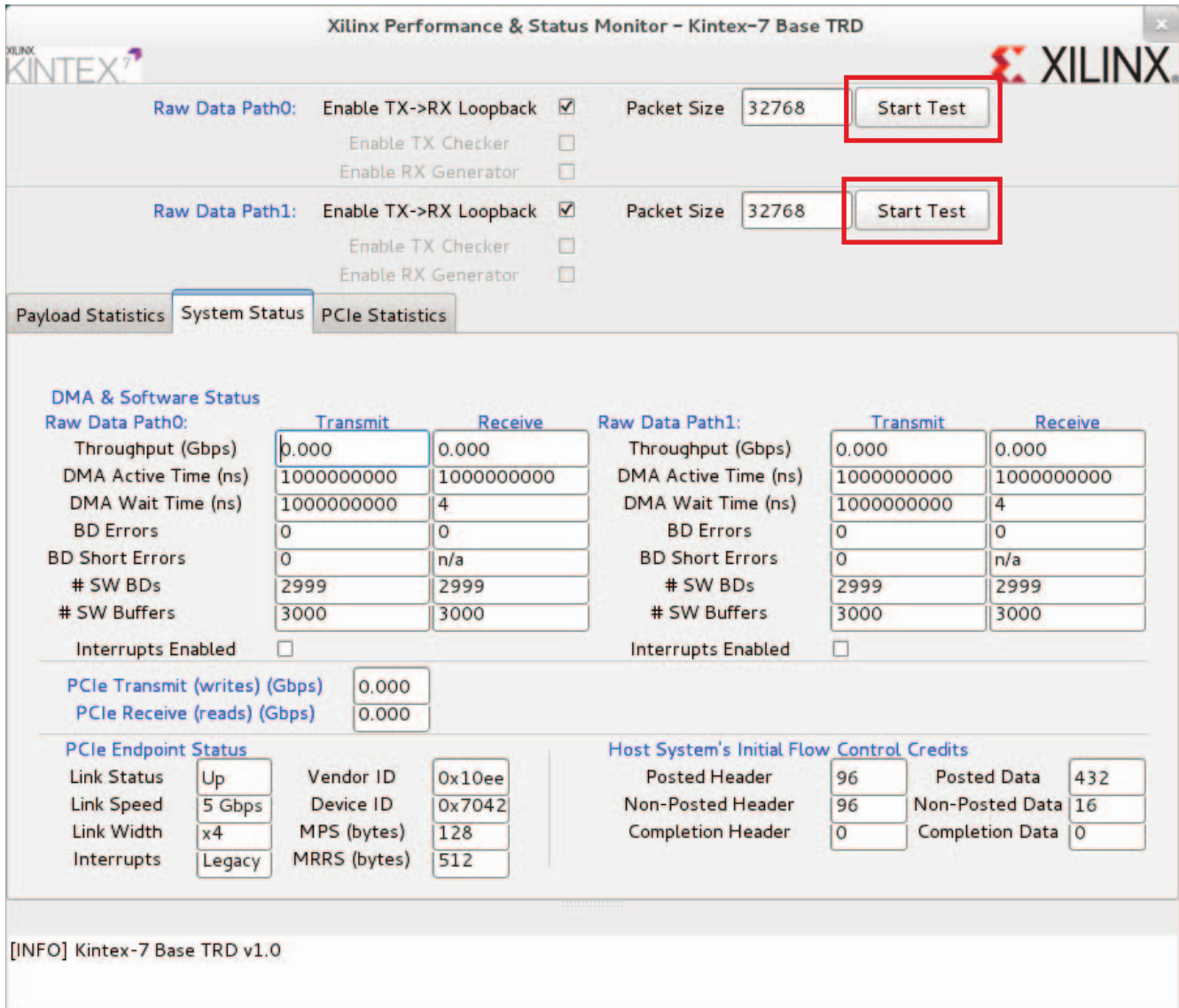
Figure 20: Start Data Traffic from the Performance Monitor
