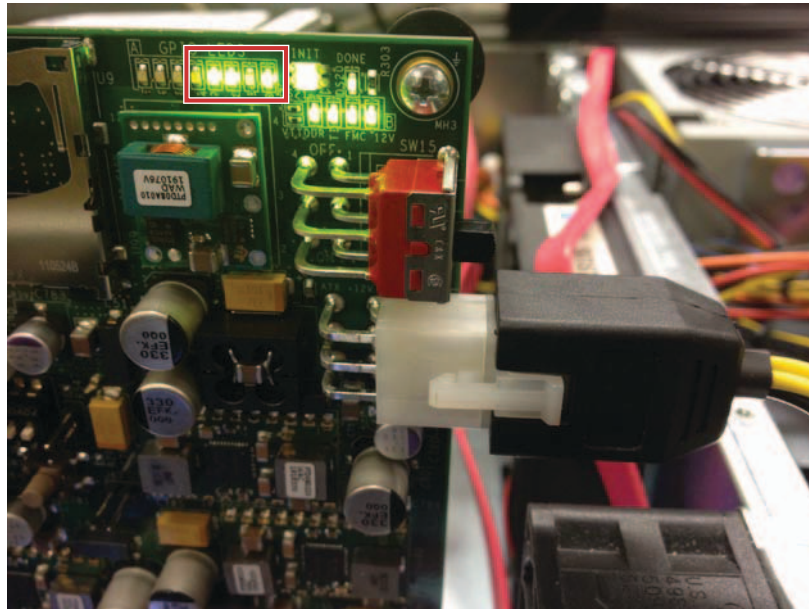
Figure 14: Location of GPIO Status LEDs (Indicates TRD Status)
