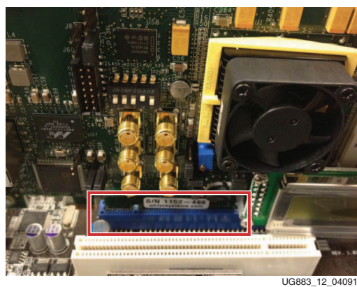
Figure 12: KC705 Board Plugged into a PCIe x16 Slot
