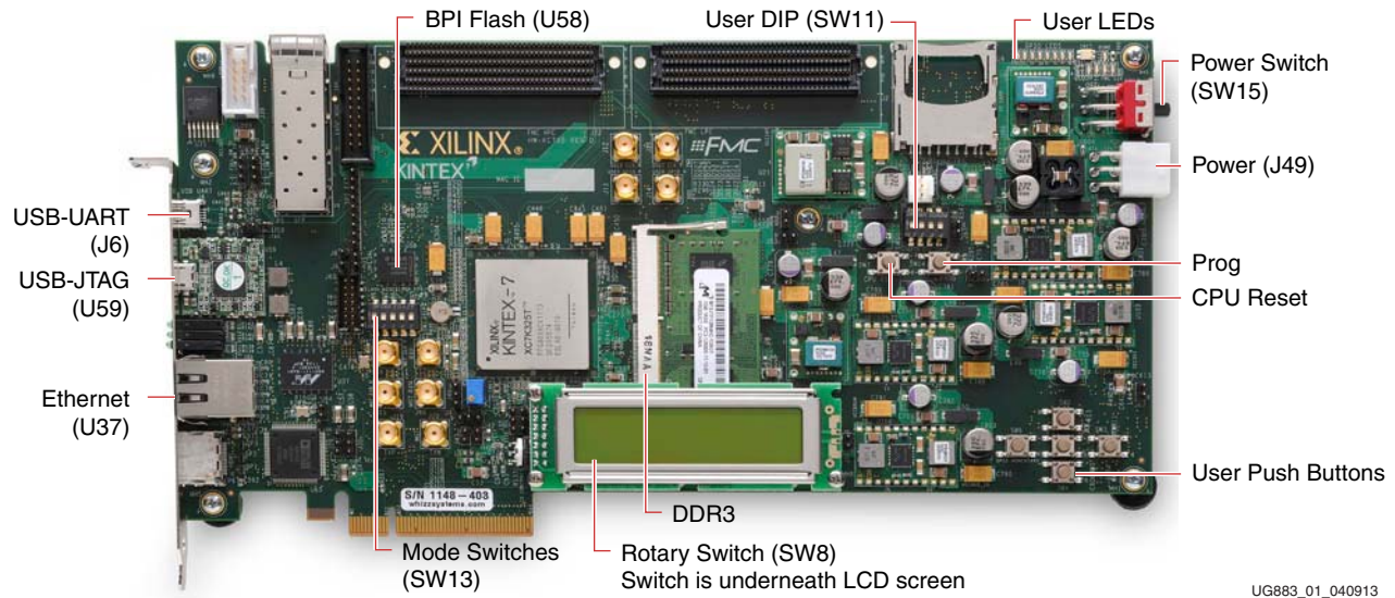
Figure 1: KC705 Board Features Used by the BIST
