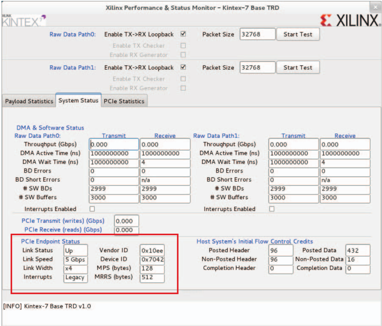
Figure 19: Verify Board Status in the Performance Monitor
