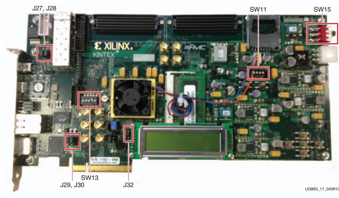
Figure 11: Switch and Jumper Settings
