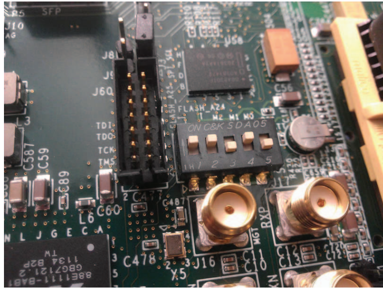
Figure 2: BIST Switch and Jumper Settings
