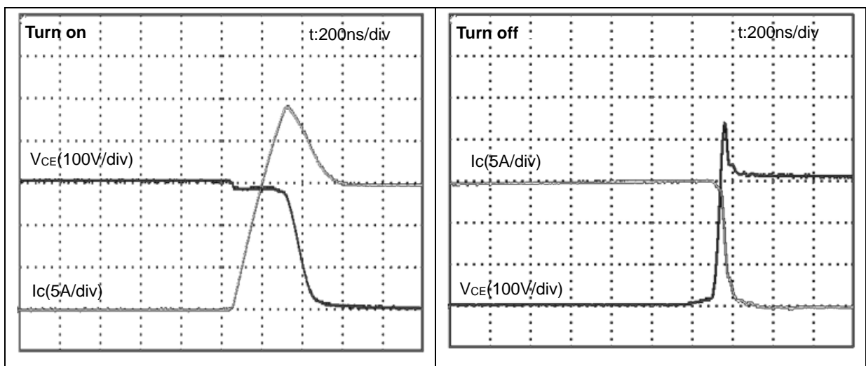
Fig.2-1-7 Typical switching waveform (SLIMDIP-L)
