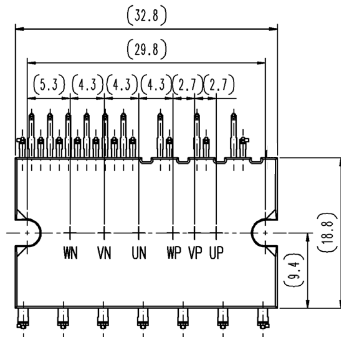
Fig.2-1-3 Power chip position
