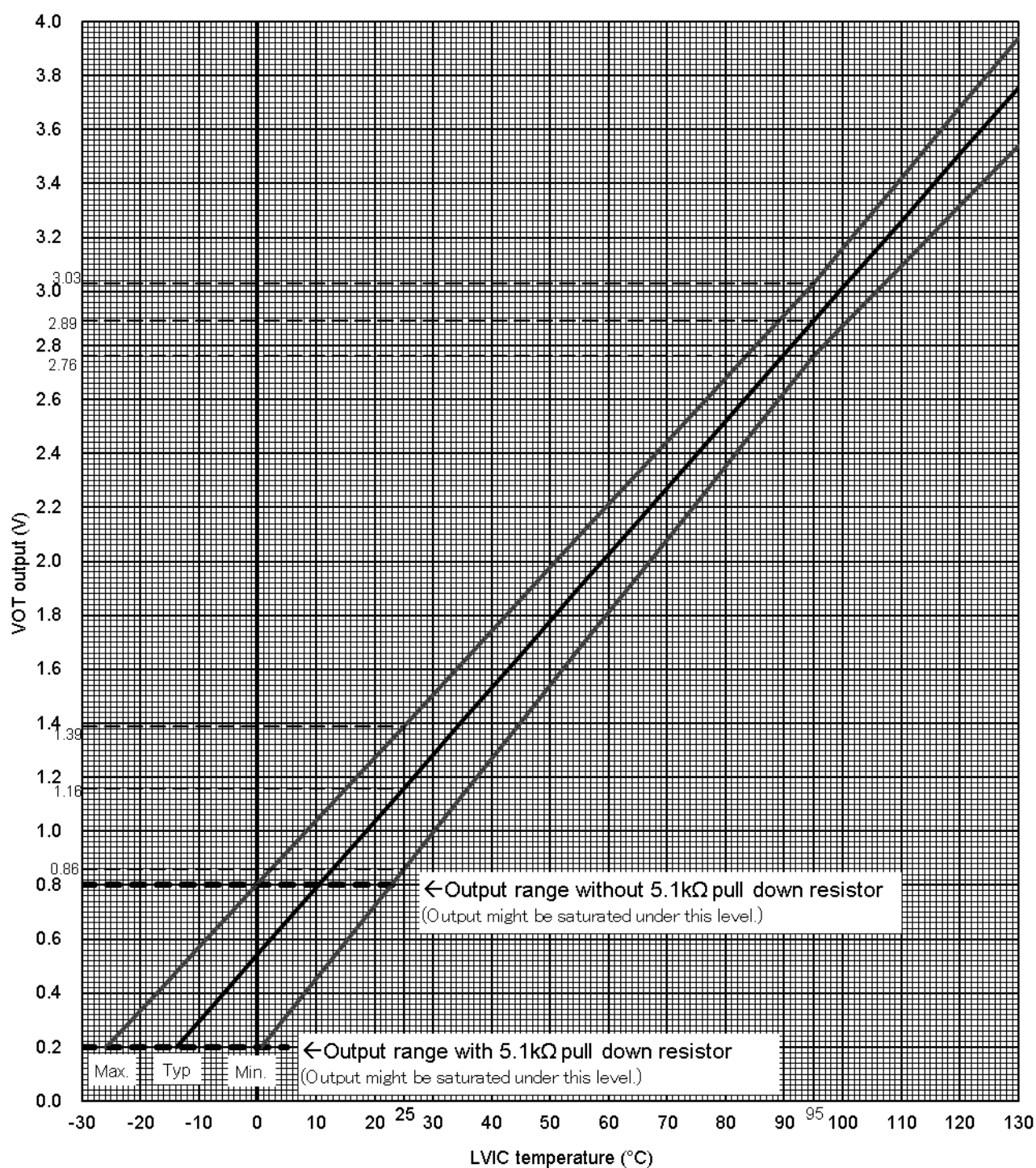
Fig.2-2-13 V_{OT} output vs. LVIC temperature
