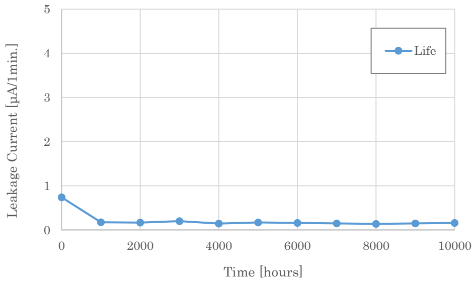
Fig. 20 Changes in leakage current with time at 105 °C (only life)
