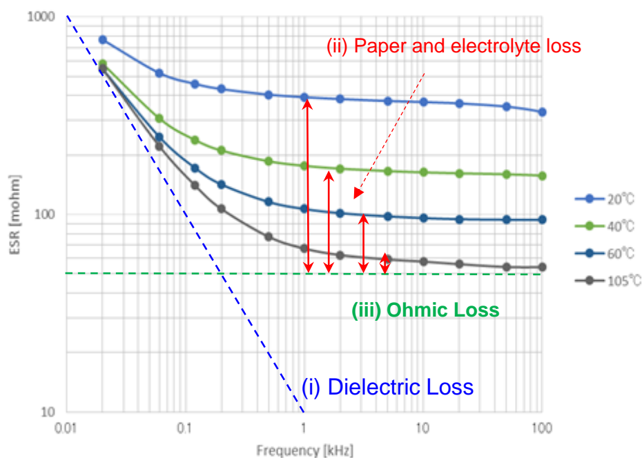
Fig. 11 ESR Characteristics of Aluminum Electrolytic Capacitor
