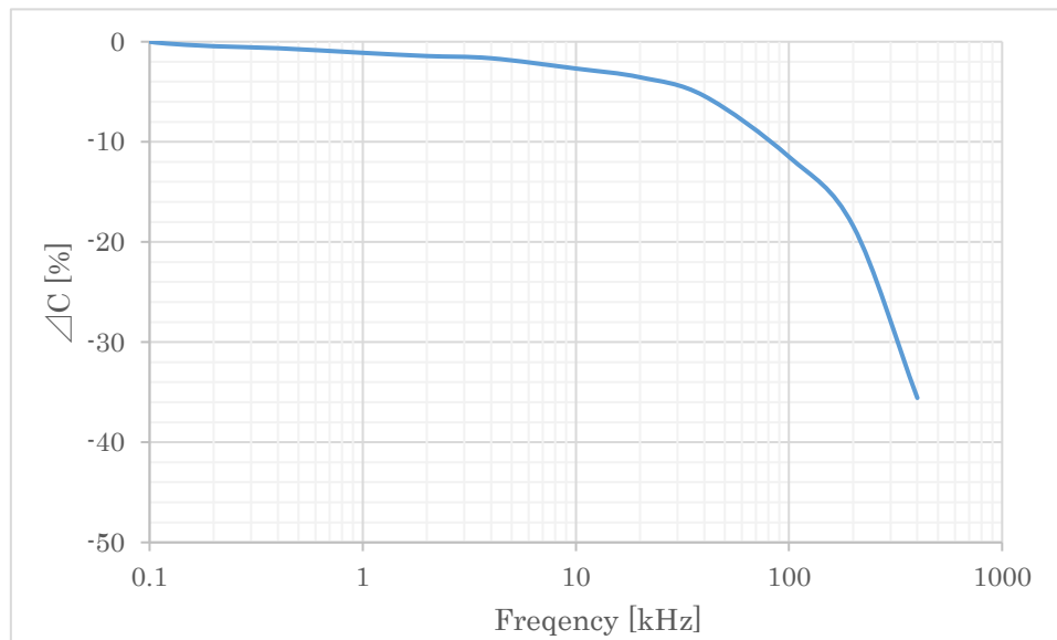
Fig. 17 The Frequency-response curve of capacitance
