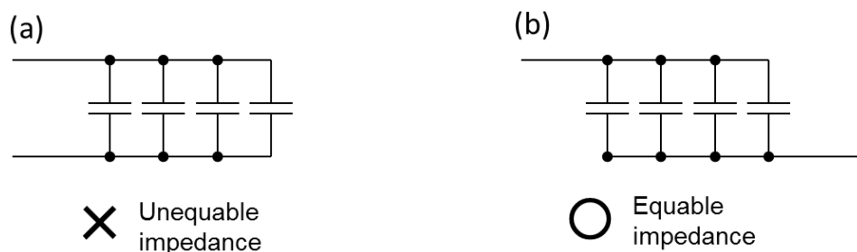
Fig. 28 Wiring for parallel connection of capacitors
