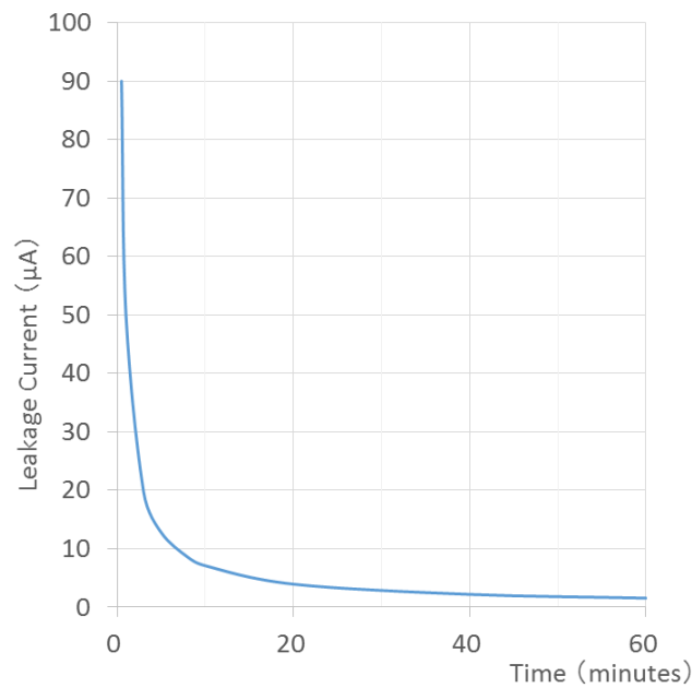
Fig. 12 Leakage current change after voltage application
