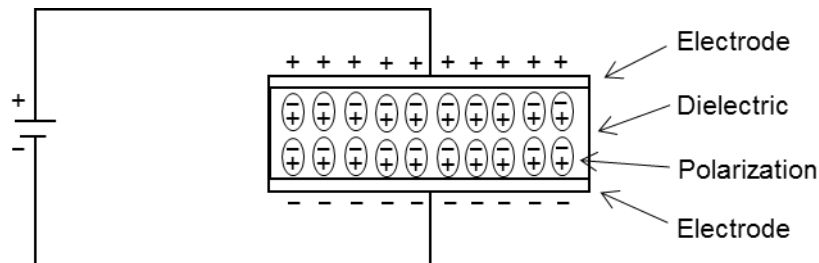
Fig. 29 Dielectric polarization during capacitor charging
