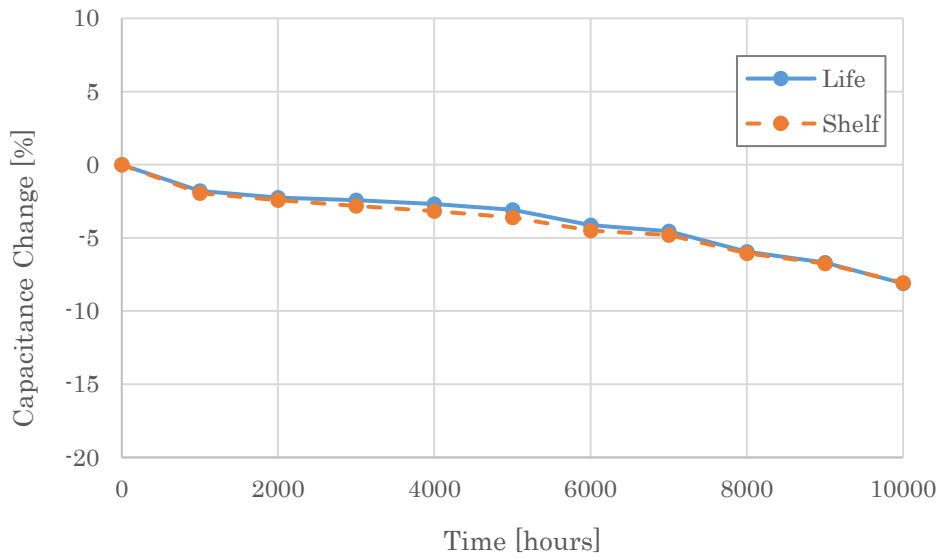
Fig. 18 Changes in capacitance with time at 105 °C
