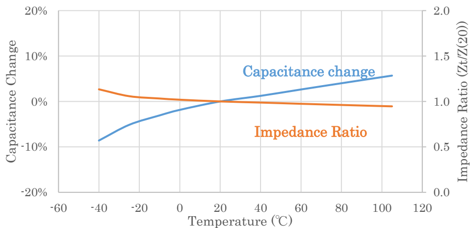
Fig. 14 Temperature Characteristics of capacitance change and impedance ratio (based on 20 °C)
