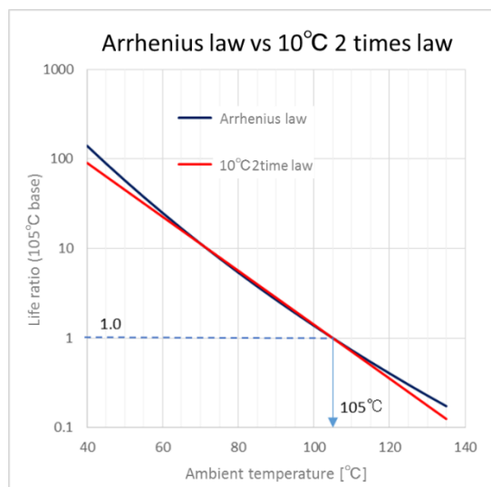
Fig. 21 Arrhenius law vs 10°C 2 times law (105°C base)
