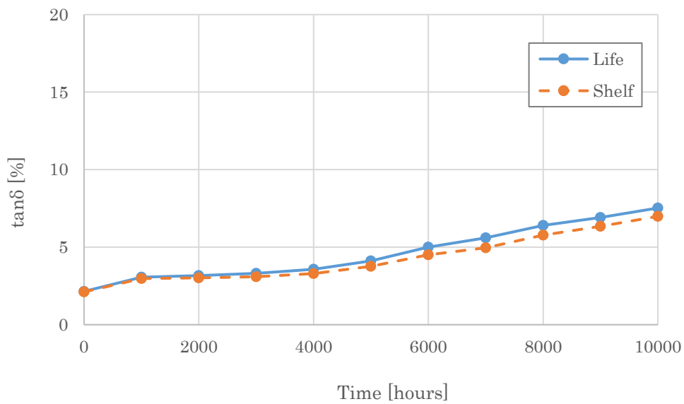
Fig. 19 Changes in tangent of loss angle ( \tan \delta ) with time at 105 °C
