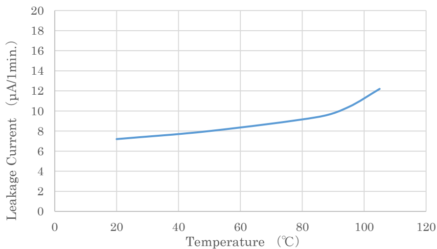
Fig. 16 Temperature Characteristics of leakage current
