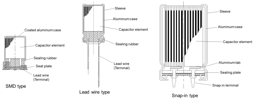
Fig. 3 Basic structure of aluminum electrolytic capacitor
