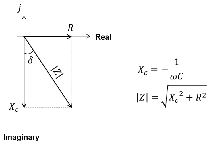
Fig. 9 Impedance and Loss angle of Capacitor
