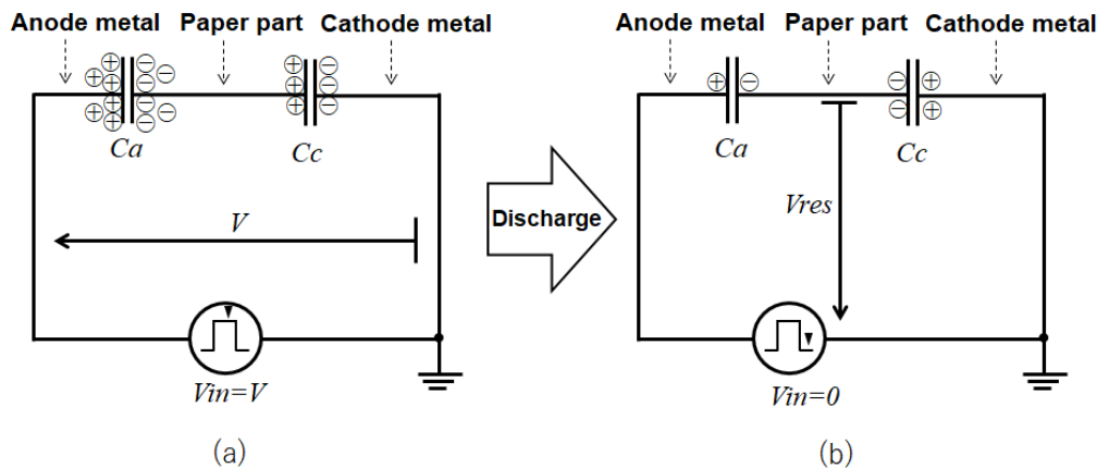
Fig. 23 The charge transformation on charge and discharge
