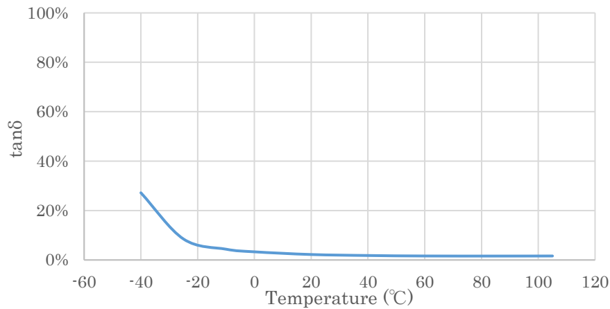
Fig. 15 Temperature Characteristics of the tangent of loss angle (tan \delta )
