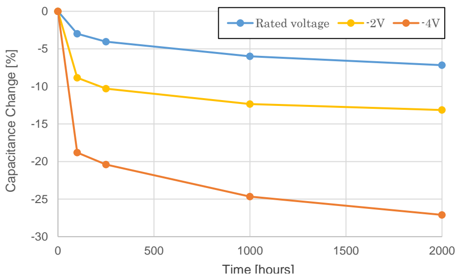
Fig. 25 Capacitance change when reverse voltage is applied
