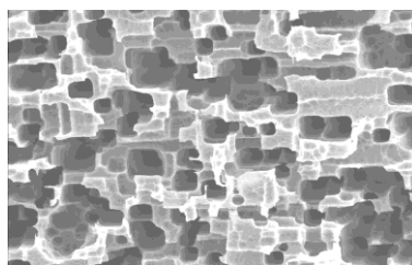
Etched foil
