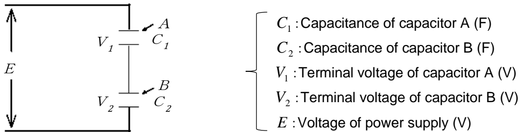
Fig. 26 Series capacitor connection
