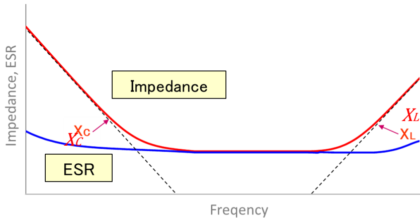
Fig. 13 Schematic illustration of impedance and ESR Frequency Characteristics
