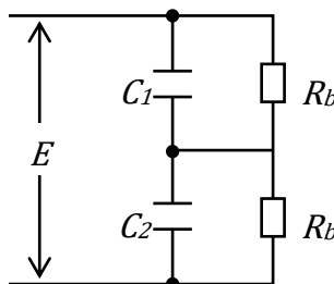
Fig. 27 Series capacitor connection with balance resistance
