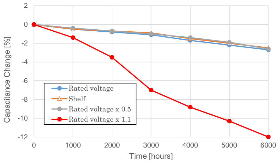
Fig. 24 Capacitance change when overvoltage is applied
