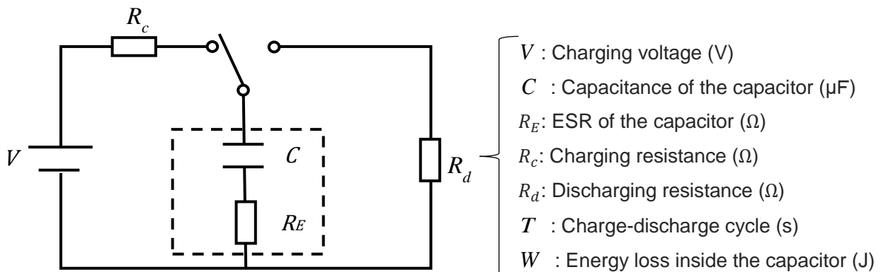
Fig. 22 Schematic diagram of charging-discharging circuit
