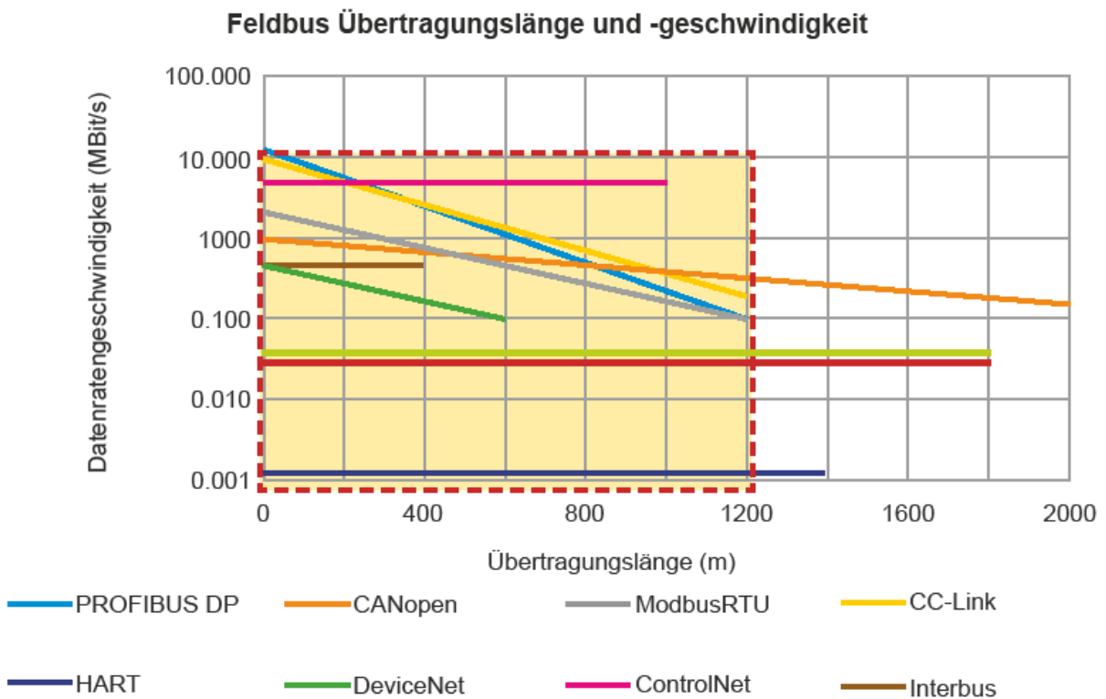
Diagram of the typical data rates and transmission lengths for popular fieldbuses (Source: IEEE 802.3 10 Mbit/s Single Twisted Pair Ethernet Call for Interest (CFI))
