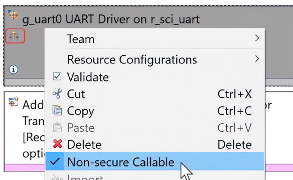
Figure 11-5: The topmost module of a stack in a secure project can be made non-secure callable
