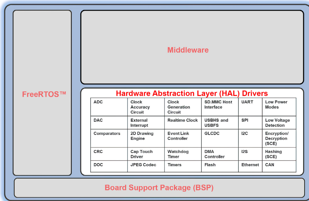
Figure 2-3: The HAL-layer provides drivers for the on-chip peripherals
