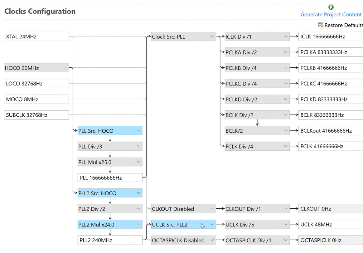
Figure 10-9: The USB FS needs a 48 MHz clock, so the clock generation circuit needs to be changed accordingly. Necessary changes are highlighted
