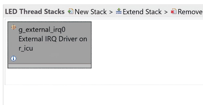
Figure 9-3: The grey color bar of the stack element indicates that this driver is a module instance and that it may be referenced by one other FSP module instance only
