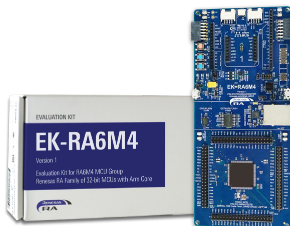
Figure 6-1: The EK-RA6M4 Evaluation Kit
