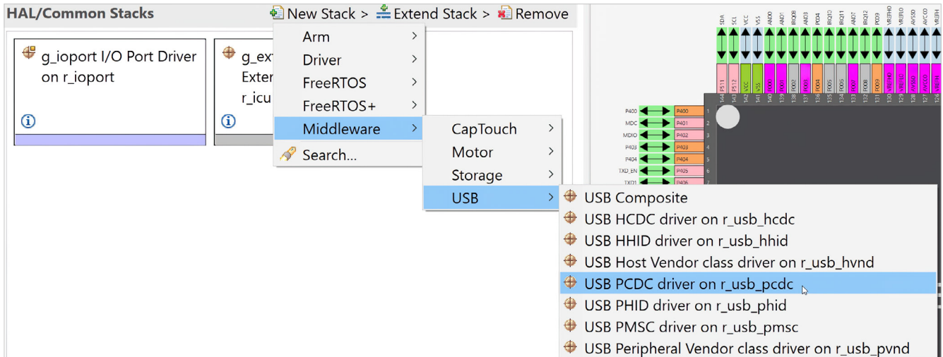
Figure 10-4: The middleware for the USB peripheral communications device class driver needs to be added to the system
