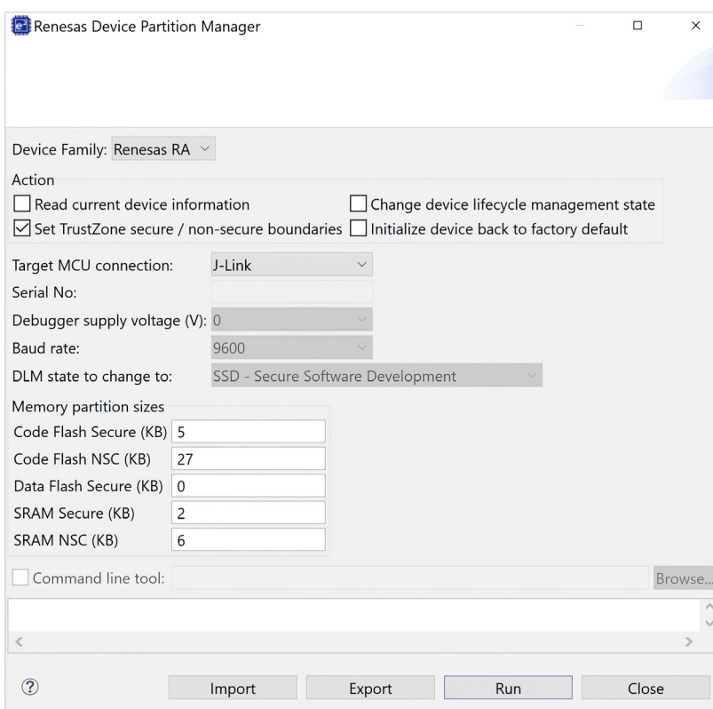
Figure 11-6: The Device Partition Manager lets you define the sizes of the different memory partitions
