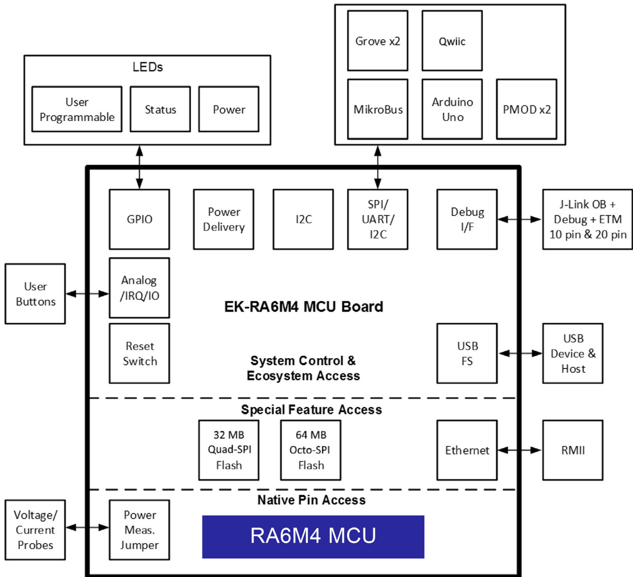
Figure 8-1: Block diagram of the EK-RA6M4 Evaluation Kit
