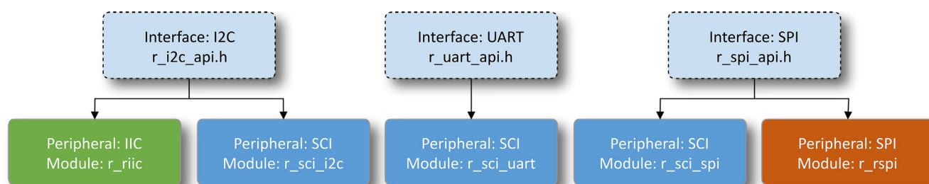
Figure 3-4: On the microcontrollers of the RA Family some peripherals will have a one-to-one mapping between the interface and instance, while others will have a one-to-many mapping
