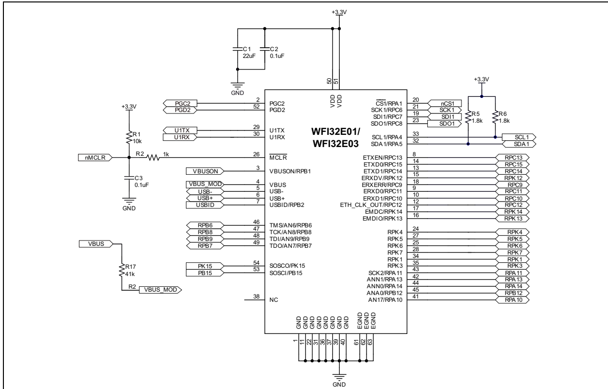
FIGURE 3-6: WFI32E01/WFI32E03 MODULE BASIC CONNECTIONS
