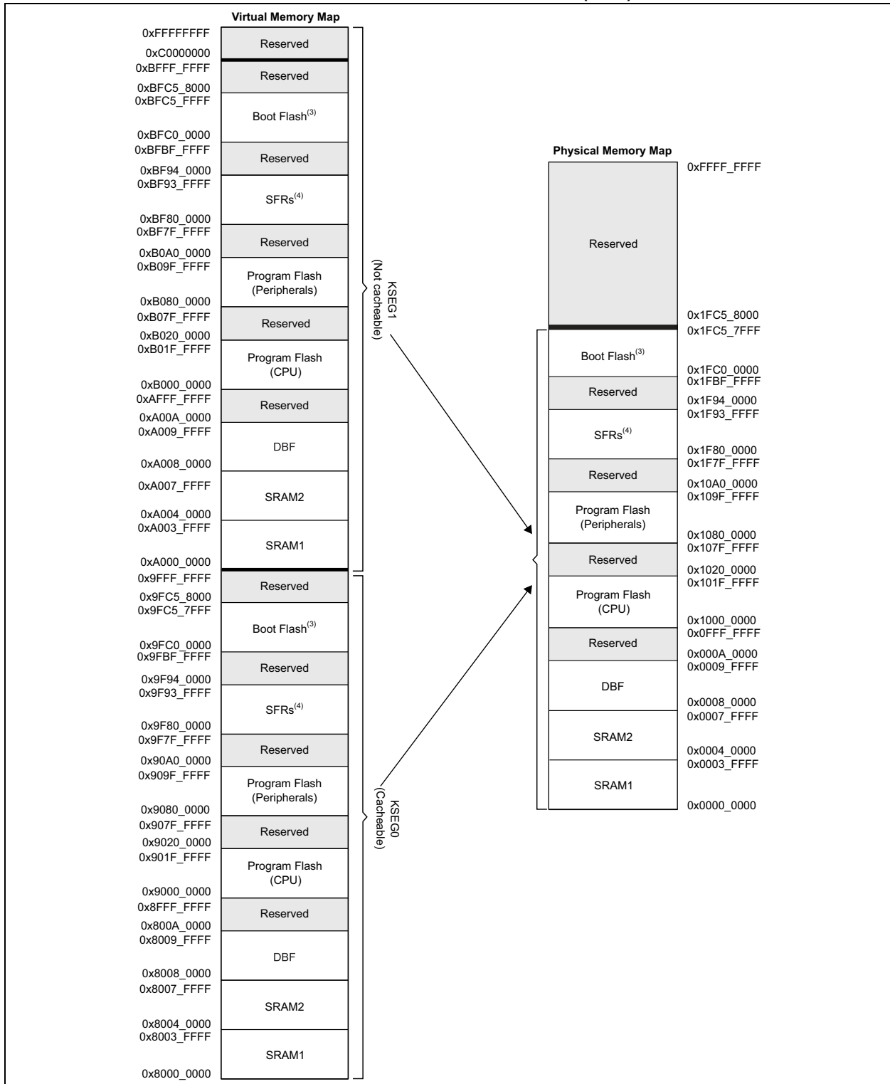
FIGURE 6-2: MEMORY MAP FOR DEVICES WITH 2048 KBYTE OF PROGRAM MEMORY, 512 KBYTE RAM AND 128 KBYTE DATA BUFFER (DBF) (1,2)
