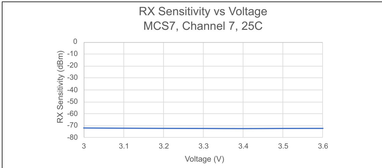
FIGURE 41-75: RX SENSITIVITY VS VOLTAGE
