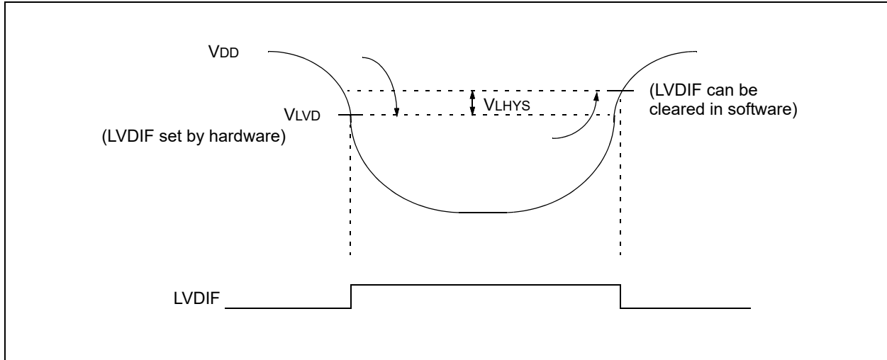
FIGURE 41-59: PROGRAMMABLE LOW-VOLTAGE DETECT ELECTRICAL CHARACTERISTICS
