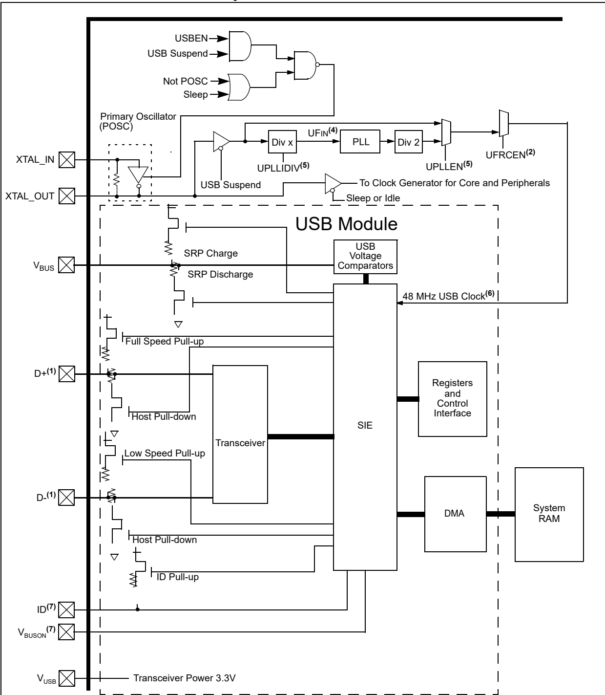
FIGURE 12-1: PIC32MZ W1 Family USB INTERFACE DIAGRAM
