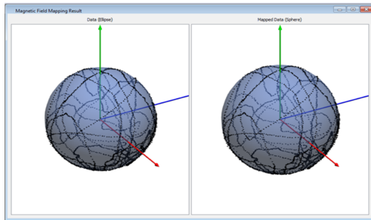
The 3D magnetic field measurements (M_x, M_y, M_z) mapped onto the surface of a sphere with its centre at (0,0,0) .
