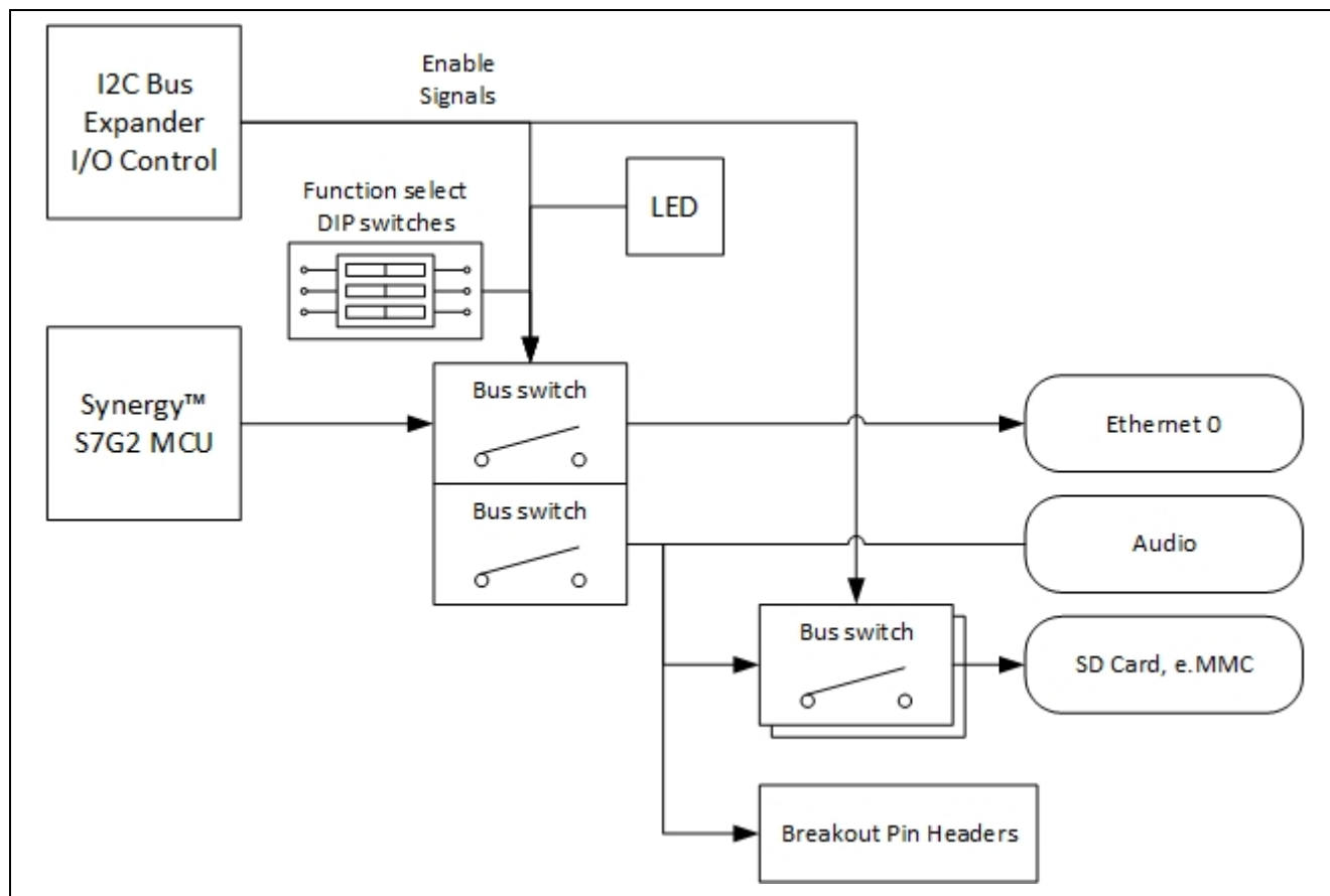
Figure 28. Ethernet 0 Multiplexing
