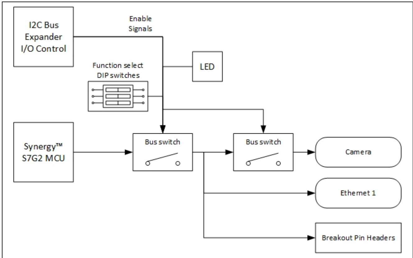
Figure 29. Ethernet 1 Multiplexing
