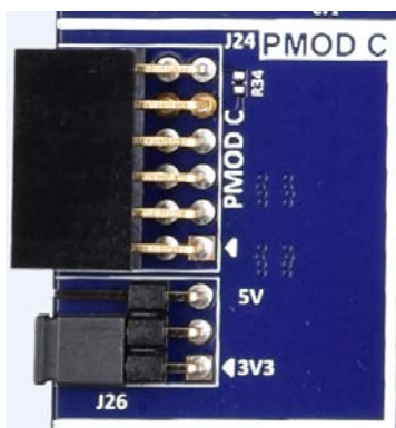
Figure 12. PMOD C
