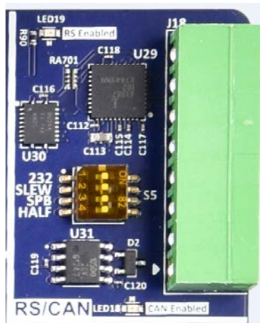
Figure 15. RS232/485 and CAN Interfaces
