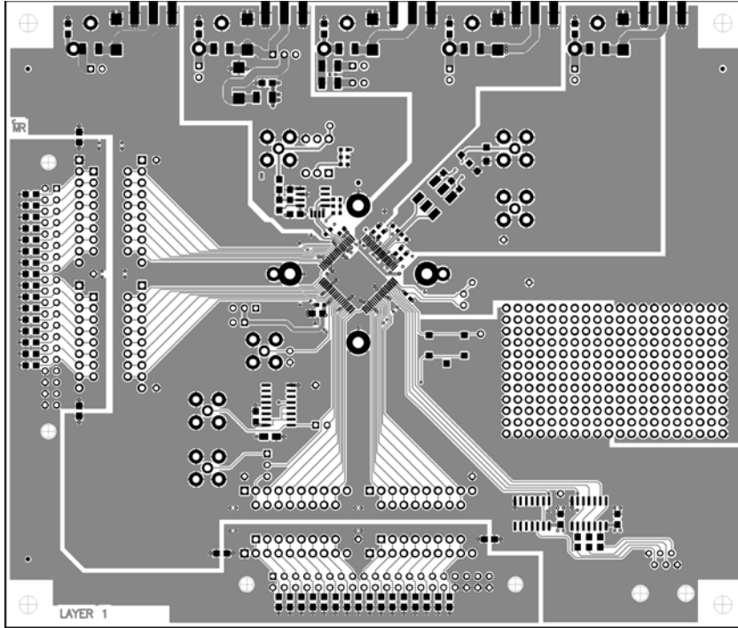
Figure 94. PCB Assembly, Layer 1 Metal, Rev. F Evaluation Board
