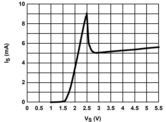
FIGURE 16. SUPPLY CURRENT vs SUPPLY VOLTAGE (PER AMPLIFIER)
