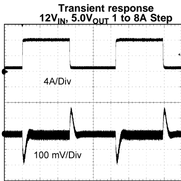
TIME (500 \mu s /Div) Figure 41.
