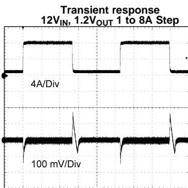
TIME (500 \mu s /Div) Figure 43.
