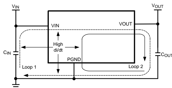
Figure 49. High Current Loops
