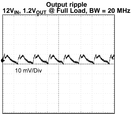
TIME (2 \mu s /Div) Figure 39.
