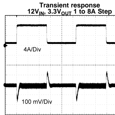
TIME (500 \mu s /Div) Figure 42.
