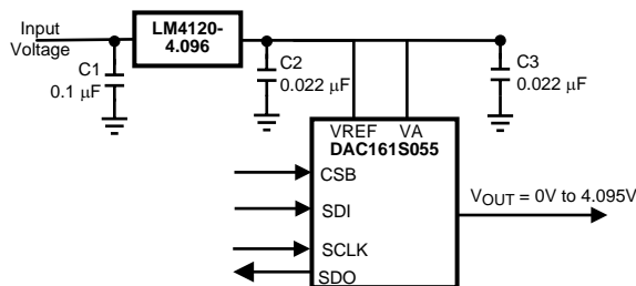
Figure 4. Using the LM4120 as a power supply
