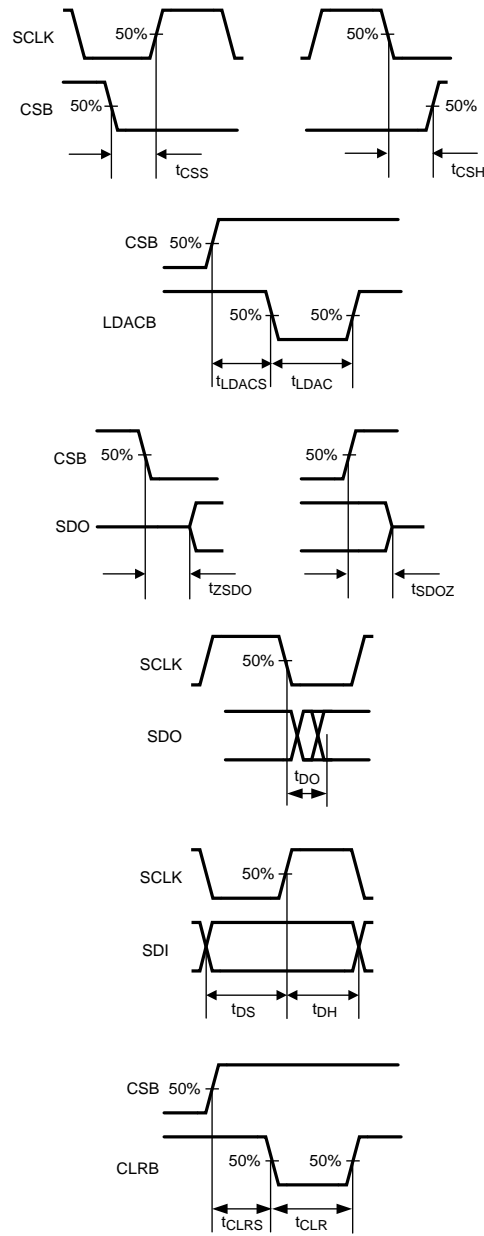
Figure 2. Timing Parameter Specifics
