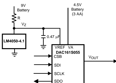
Figure 5. Using the LM4050 in a low noise circuit
