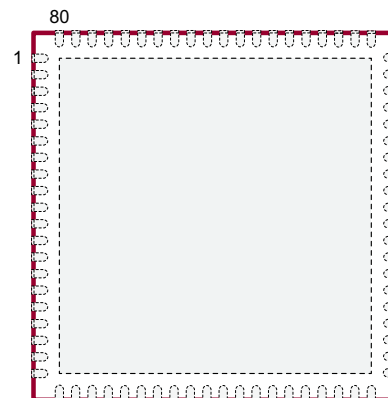
80-Lead QFN (top view)
