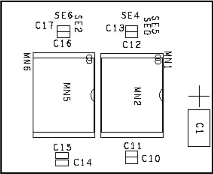
Figure 4-2. Component Side
