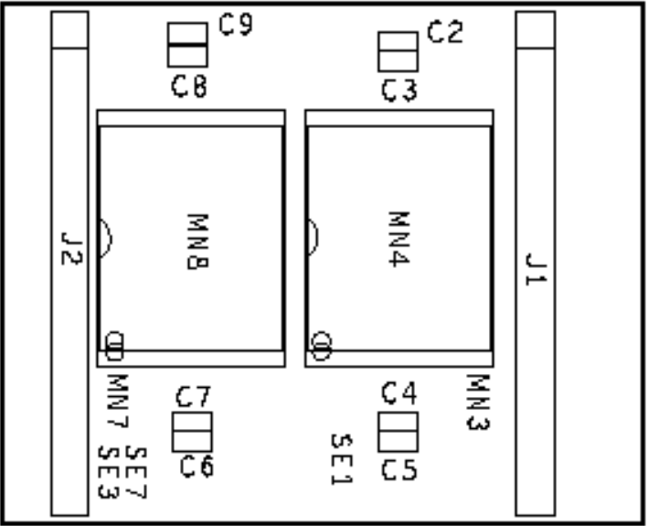
Figure 4-3. Solder Side
