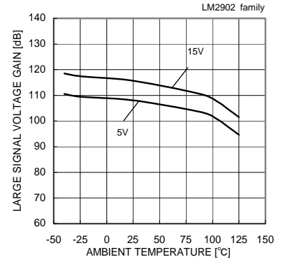
Fig. 93 Large Signal Voltage Gain – Ambient Temperature (RL=2[kΩ])
