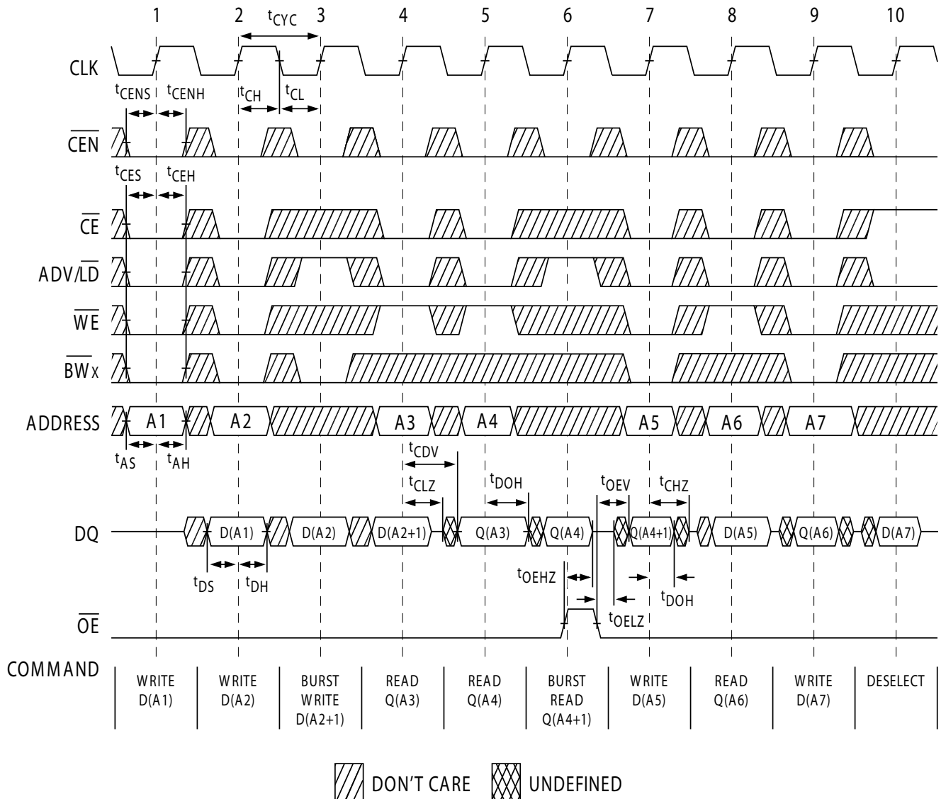
Figure 7. Read/Write Waveforms [28, 29, 30]
