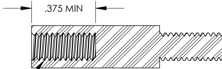
SECTION A-A 8-32 THREADS
