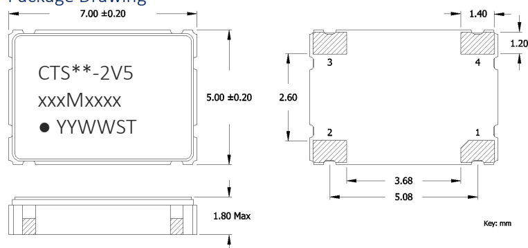
Package Drawing
