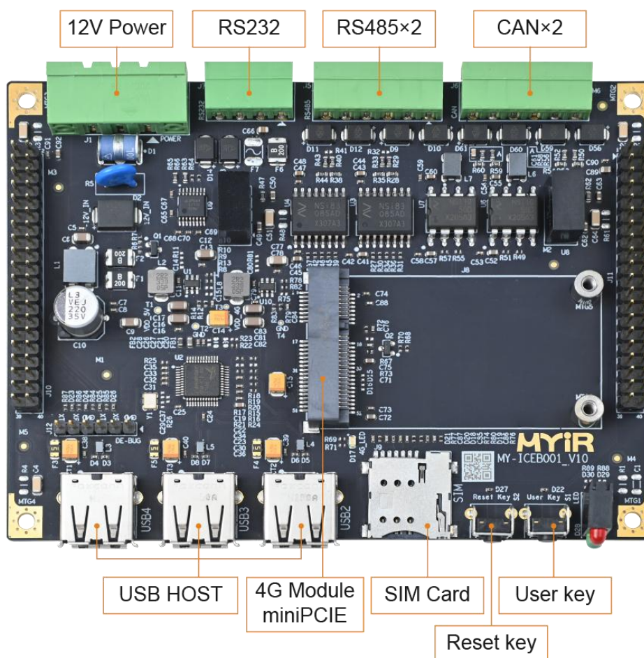
MY-ICEB001 Expansion Board
