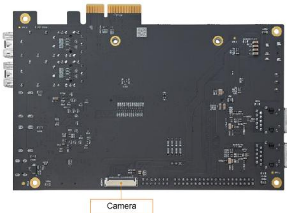
MYD-J7A100T Development Board Bottom-view
