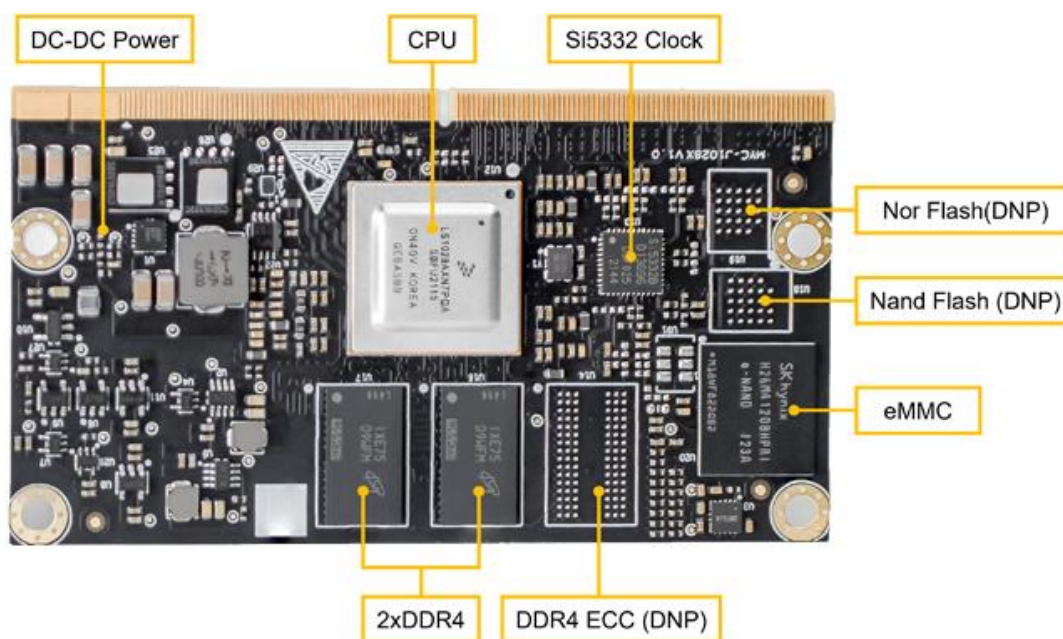
MYC-J1028X Top-view
