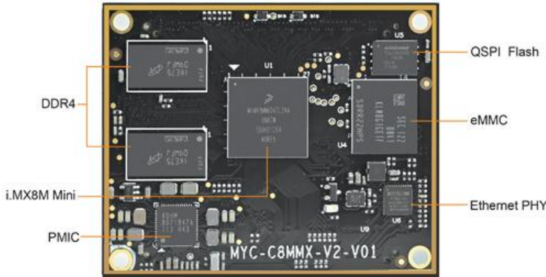
MYC-C8MMX-V2 Top-view
