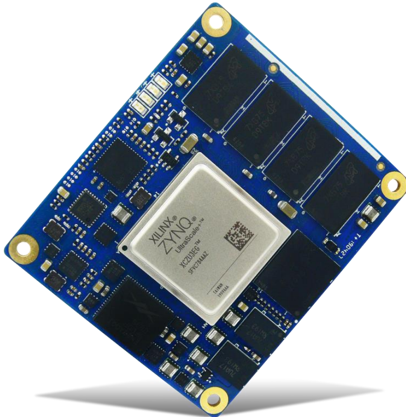
Figure 1-1 MYC-CZU3EG/4EV CPU Module
