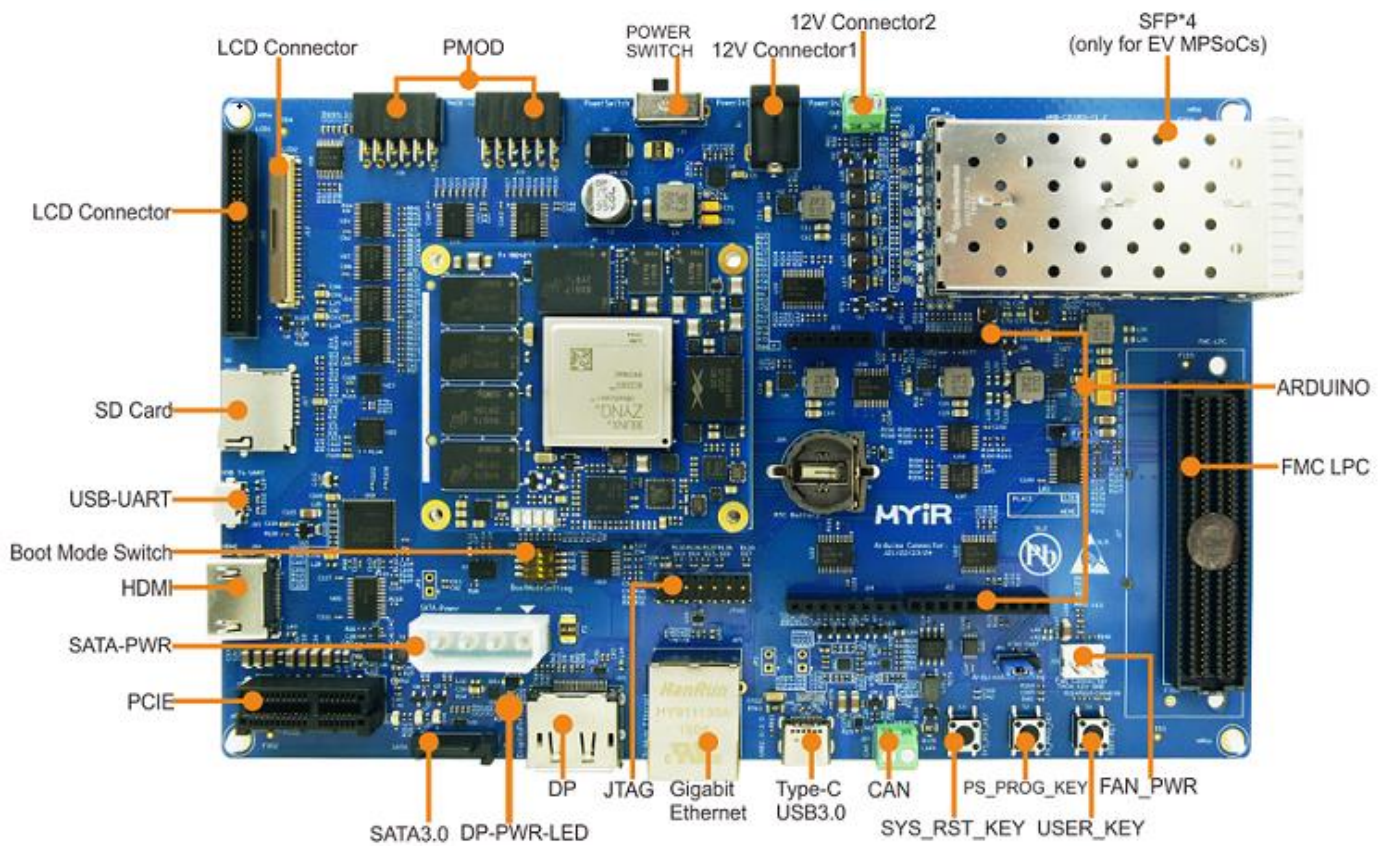
Figure 1-3 MYD-CZU3EG/4EV Development Board
