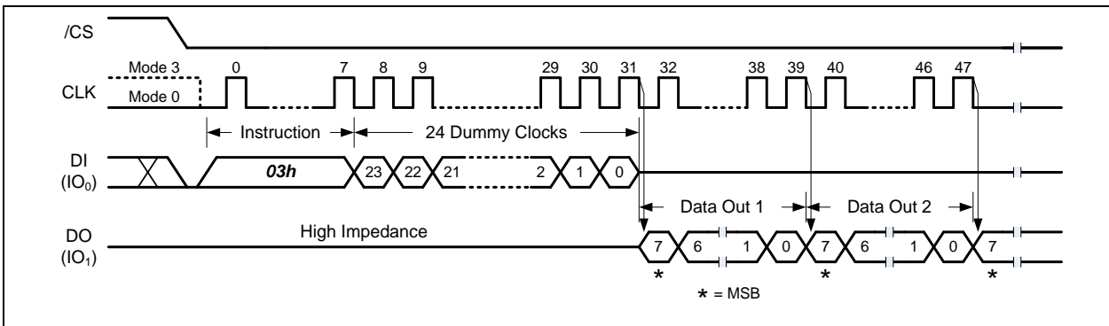
Figure 26. Read Data Instruction (Continuous Read Mode, BUF=0)
