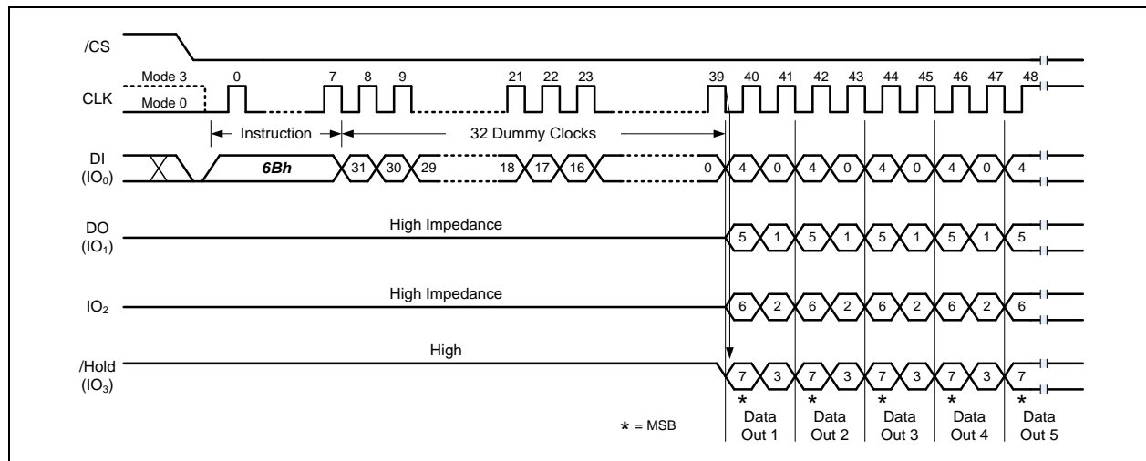
Figure 32. Fast Read Quad Output Instruction (Continuous Read Mode, BUF=0)
