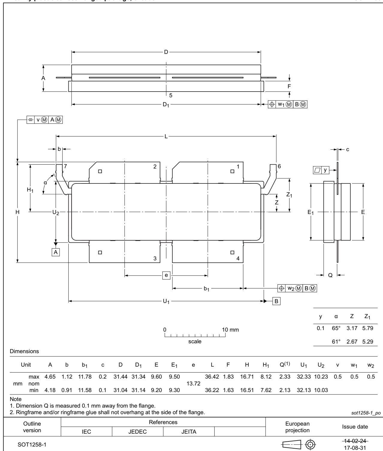
Fig 8. Package outline SOT1258-1
