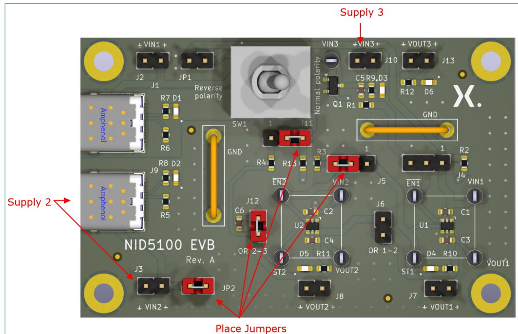
Fig. 11. Board setup for OR-ing between supply 2 and supply 3 using a PMOST
