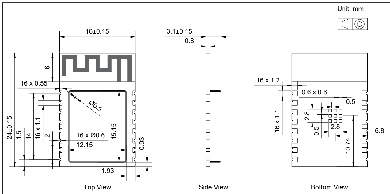
Figure 6: Physical Dimensions
