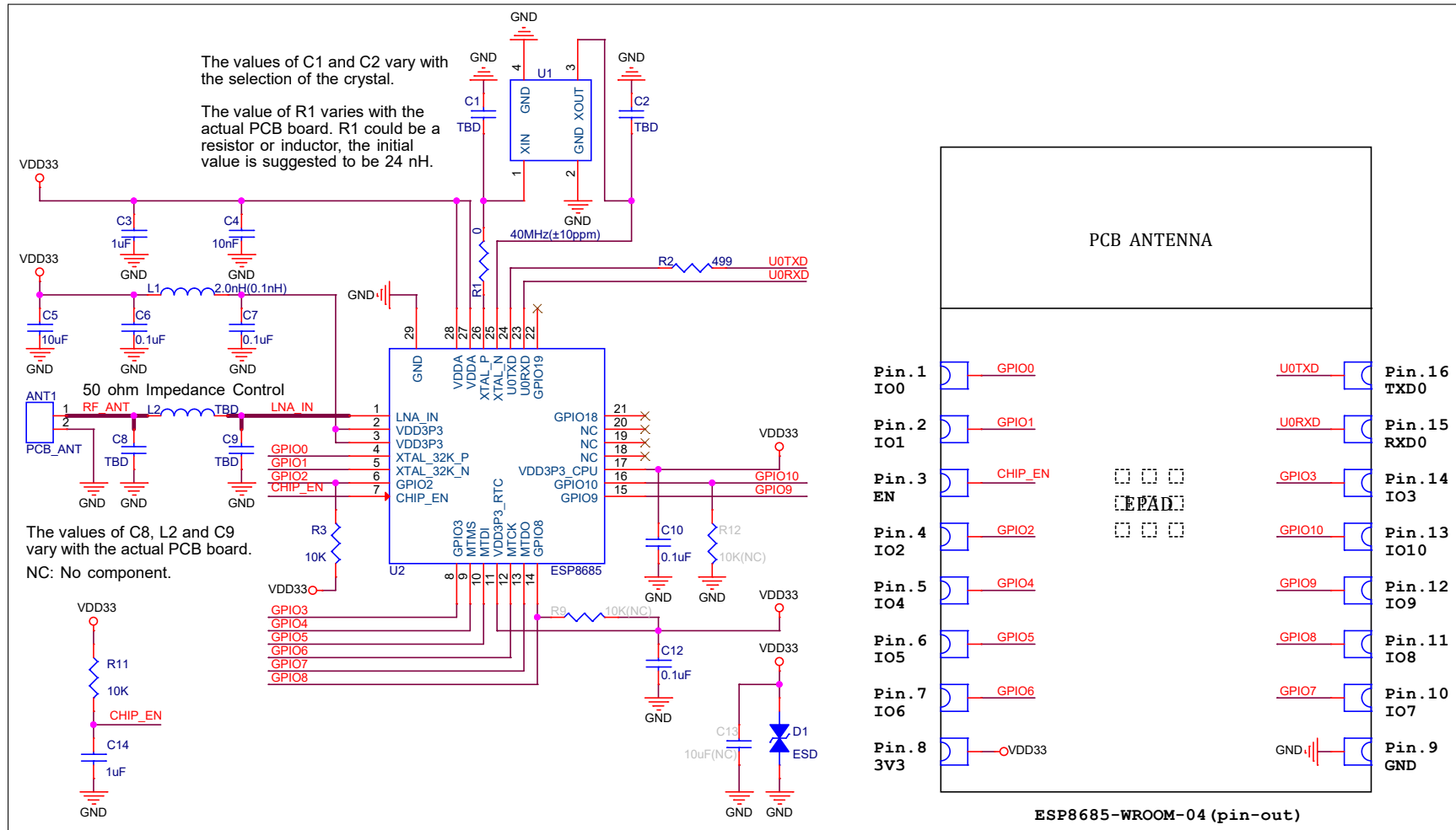
Figure 4: Schematics
