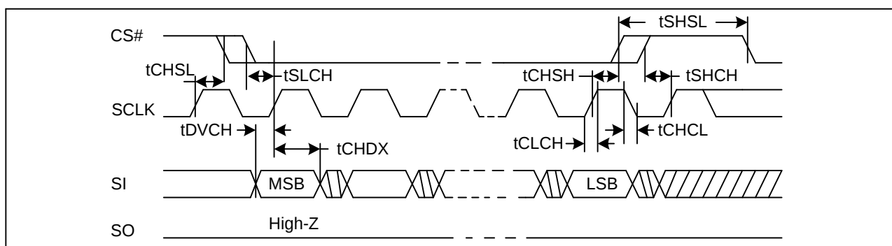
Figure 44. Input Timing
