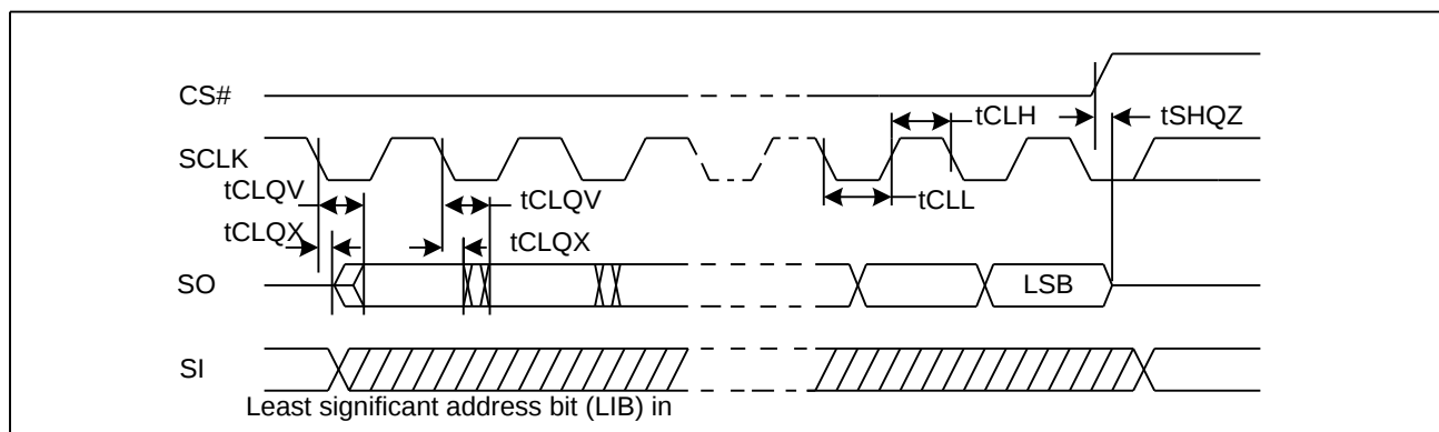
Figure 45. Output Timing
