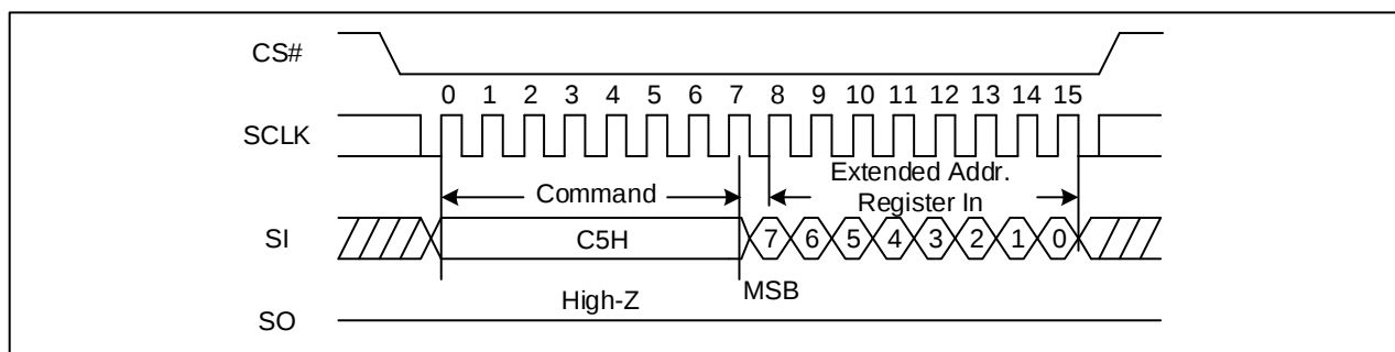
Figure 10 Write Extended Address Register Sequence Diagram
