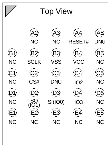
Figure 3 Connection Diagram for TFBGA24 package
