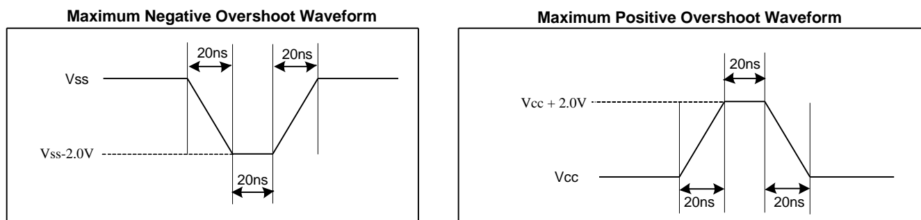
Figure 14. Overshoot Waveform
