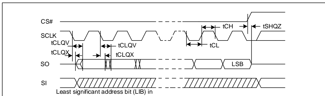
Figure 18-2. Serial Output Timing
