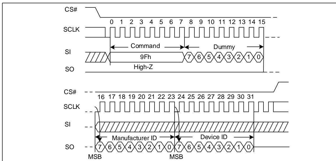
Figure 8-8. Read ID Sequence Diagram
