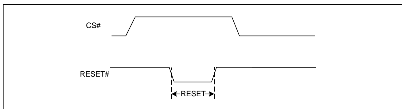
Figure 4 RESET Condition
