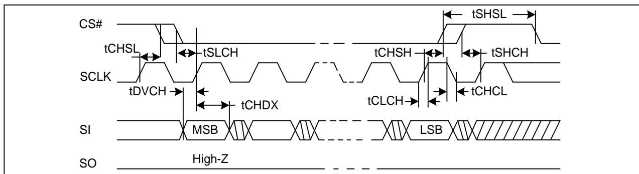
Figure 44. Input Timing
