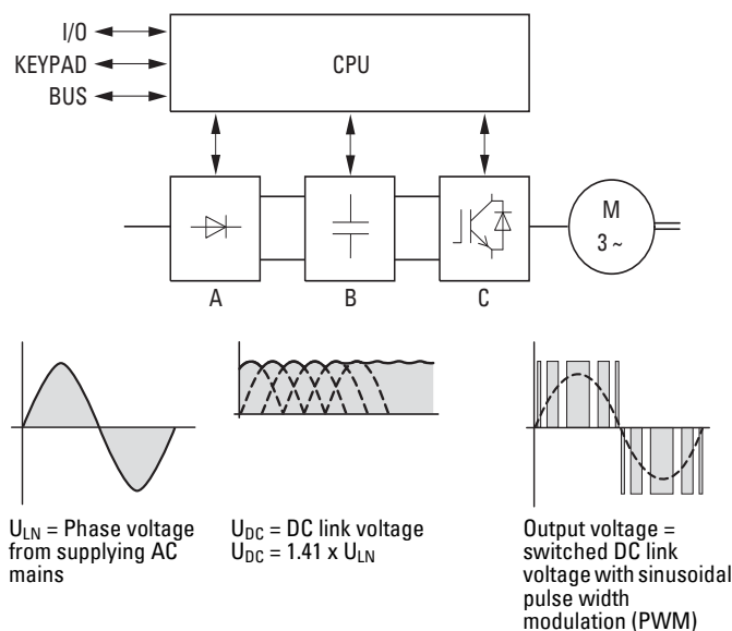
Block diagram with main components of a variable frequency drive
