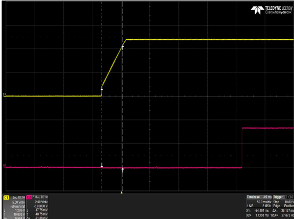
Figure 7: DS1100SLPE-3 Output Voltage Startup - V_{in} = 115V_{ac} Full Load: I_o = 90.0A Ch 1: V_o Ch 2: PWOK
