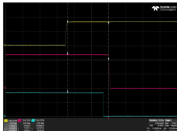
Figure 10: DS1100SLPE-3 Turn Off Characteristic via PS_ON_L Full Load: I_o = 90.0A Ch 1: PS_ON_L Ch 2: V_o Ch 3: PWOK
