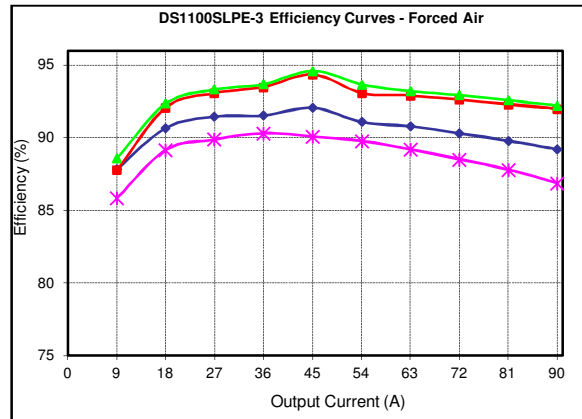
Figure 16: DS1100SLPE-3 Efficiency Curves @ 25 degC * 90 Vac * 115 Vac * 230 Vac * 264 Vac Loading: I_o = 10\% I_{o,max} increment to 90.0A
