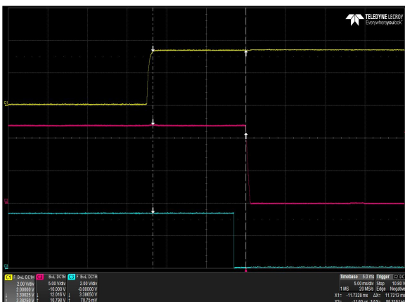
Figure 11: DS1100SLPE-3 Turn Off Characteristic via PS_KILL_L Full Load: I_o = 90.0A Ch 1: PS_KILL_L Ch 2: V_o Ch 3: PWOK
