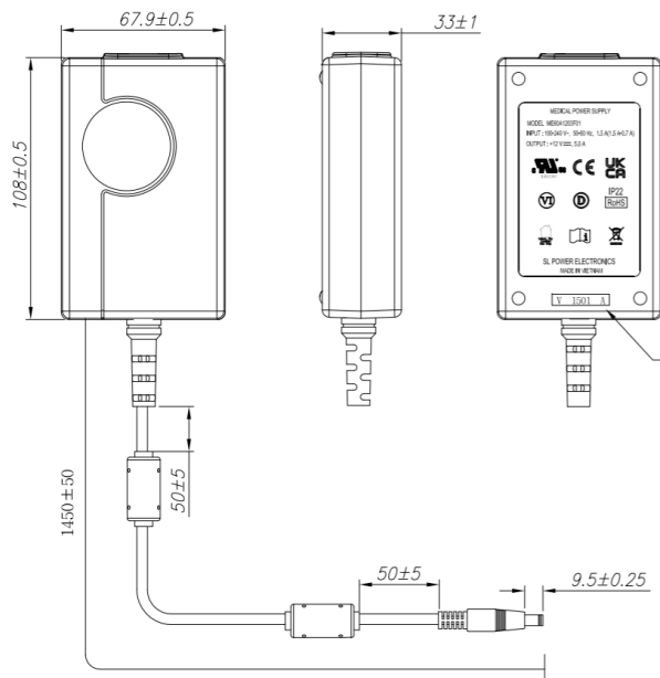
9V through 48V Models: 2.5mm x 5.5mm x 9.5mm or equiv, Barrel Connector, center positive 2
