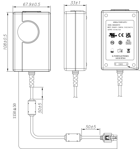
5V Models Output Connector: 6 pin Molex 39-01-2060 or equiv. Pins 1,4 = (+), Pins 3,6 = (-), Pins 2,5 = NC 2
