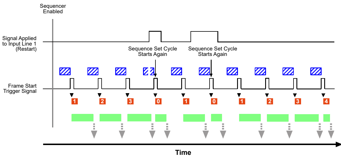
Fig. 58: Sequencer in Controlled Sequence Advance Mode with Always Active as the Sequence Control Source and Synchronous Restart Controlled by Line 1
