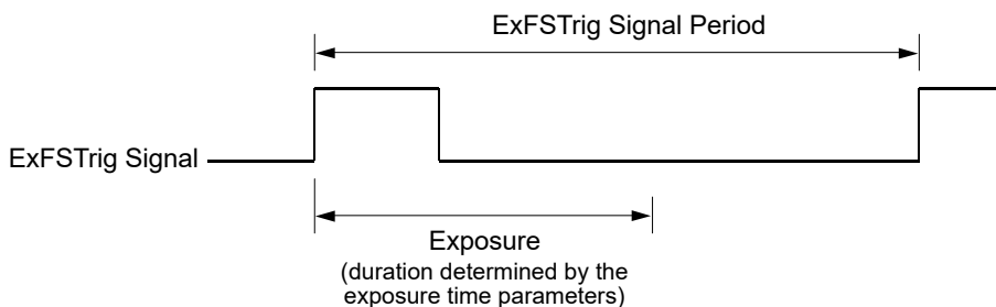
Fig. 32: Timed Exposure with Rising Edge Triggering
