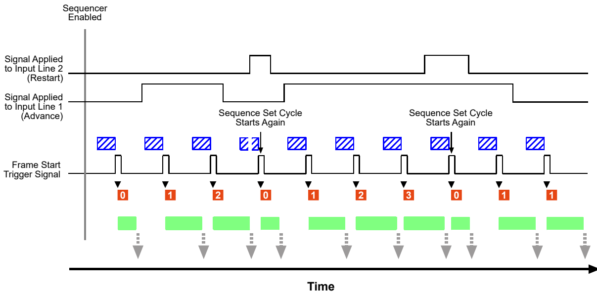
Fig. 60: Sequencer in Controlled Sequence Advance Mode with Line 1 as the Sequence Control Source and Synchronous Restart Controlled by Line 2
