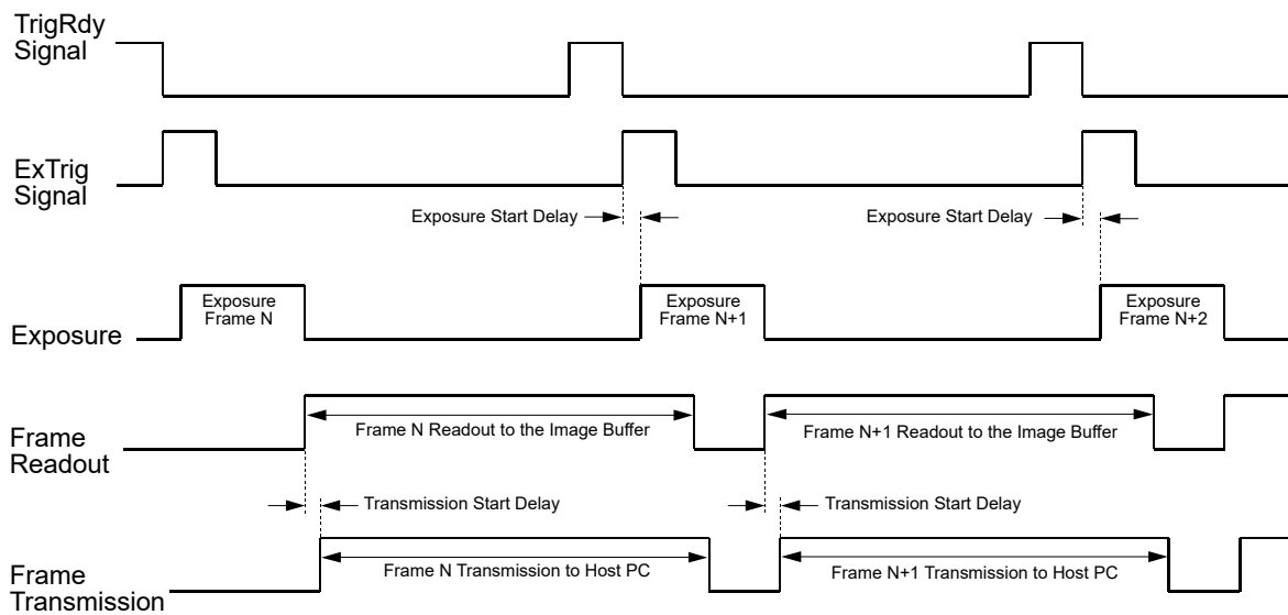
Fig. 49: Exposure Start Controlled with an ExTrig Signal
