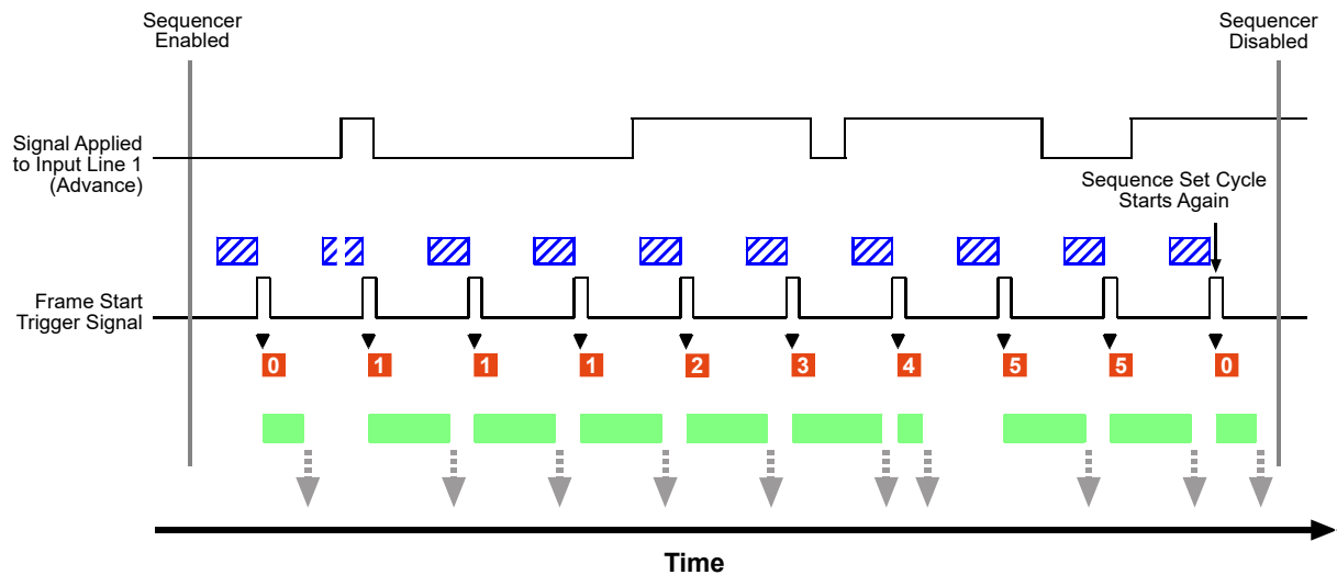
Fig. 59: Sequencer in Controlled Sequence Advance Mode with Line 1 as the Sequence Control Source
