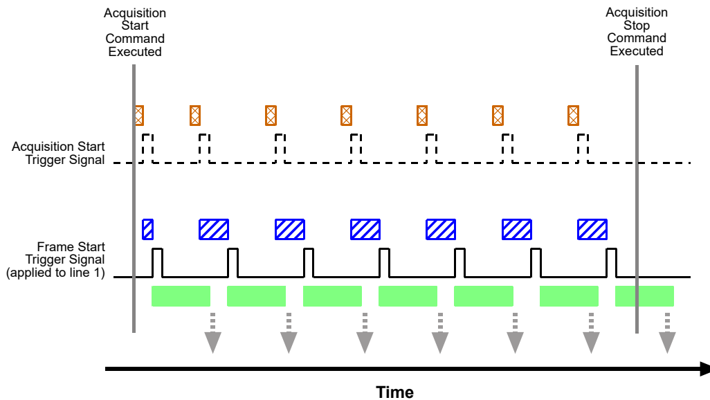
Fig. 41: Use Case 2 - Acquisition Start Trigger Off and Frame Start Trigger On
