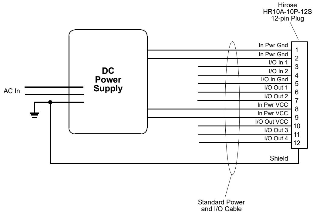
Fig. 22: Standard Power and I/O Cable
