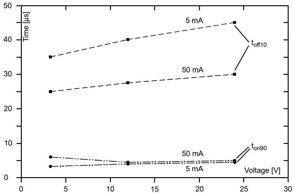
Fig. 26: Dependence of t_{on90} and t_{off10} on Voltage, for Different Load Currents; Measured for an Individual Camera as an Example
