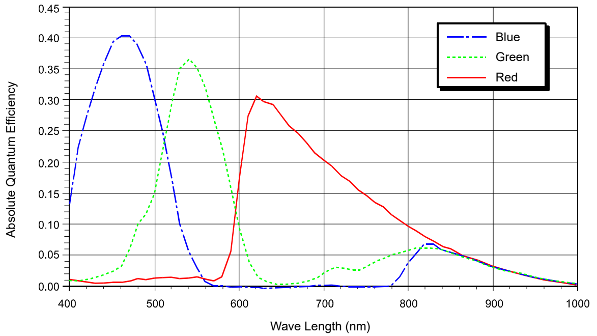
Fig. 7: piA1600-35gc Spectral Response
