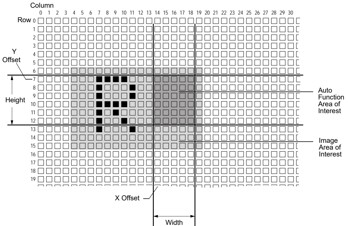
Fig. 69: Auto Function Area of Interest and Image Area of Interest
