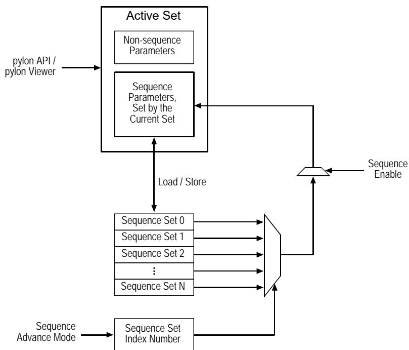
Fig. 55: Sequence Feature Block Diagram
