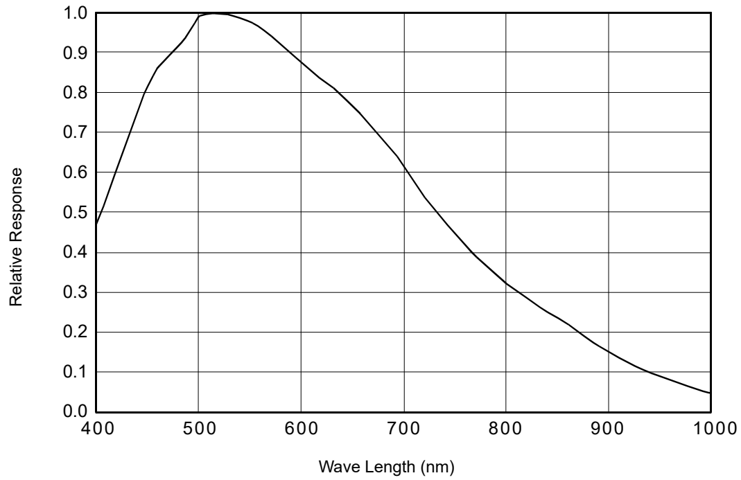
Fig. 4: piA2400-17gm Spectral Response
