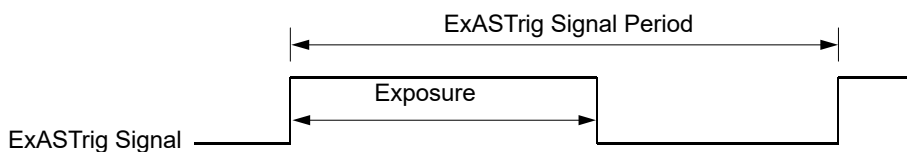
Fig. 38: Trigger Width Exposure with Rising Edge Triggering
