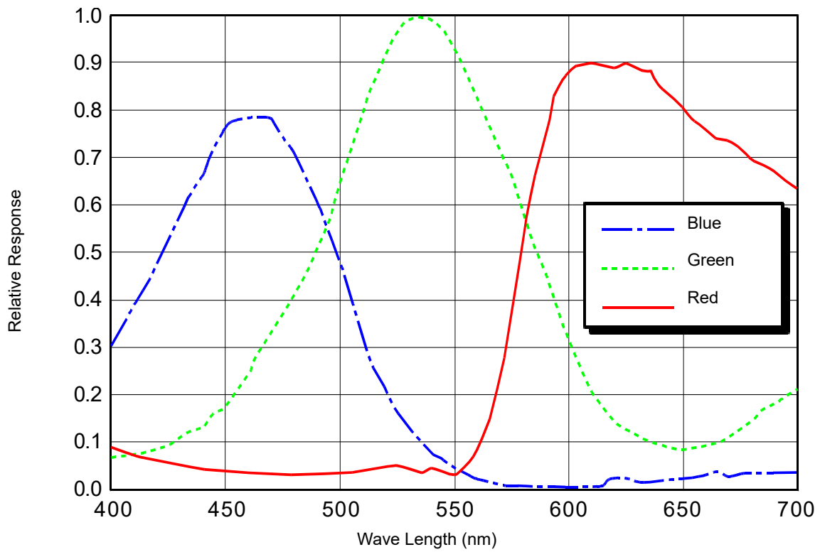
Fig. 8: piA2400-17gc Spectral Response
