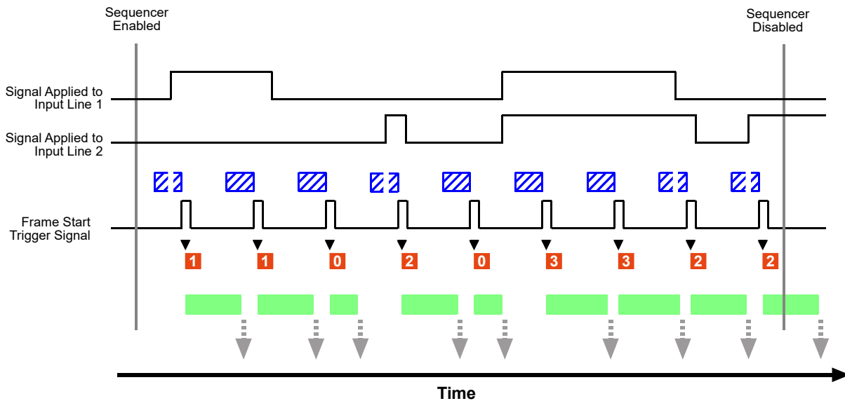
Fig. 62: Sequencer in Free Selection Mode
