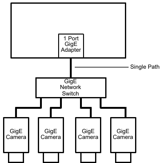
Fig. 17: Multiple Cameras on a Network
