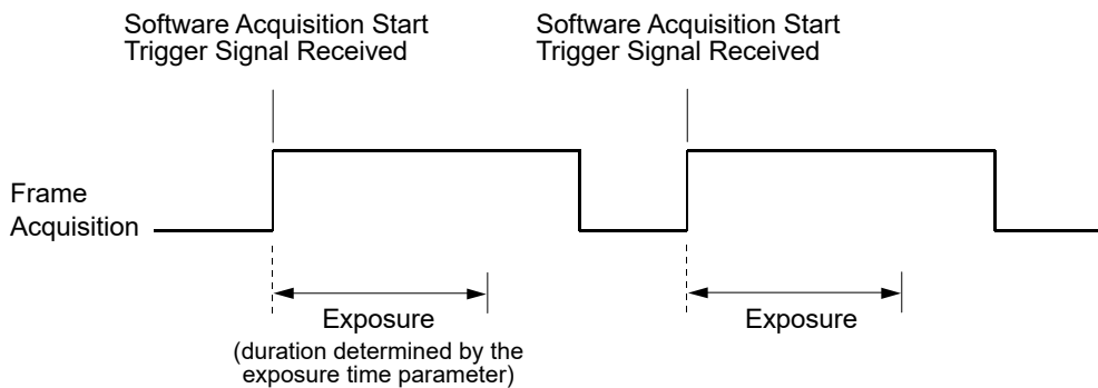
Fig. 35: Frame Acquisition with a Software Acquisition Start Trigger
