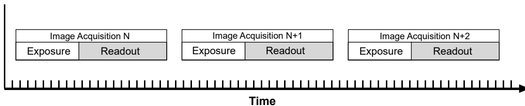
Fig. 44: Non-overlapped Exposure
