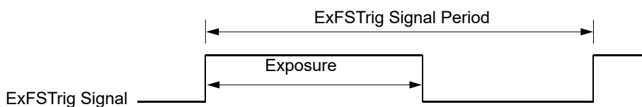
Fig. 34: Trigger Width Exposure with Rising Edge Triggering
