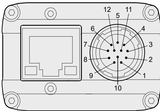
Fig. 21: Pin Numbering for the 12-pin Receptacle
