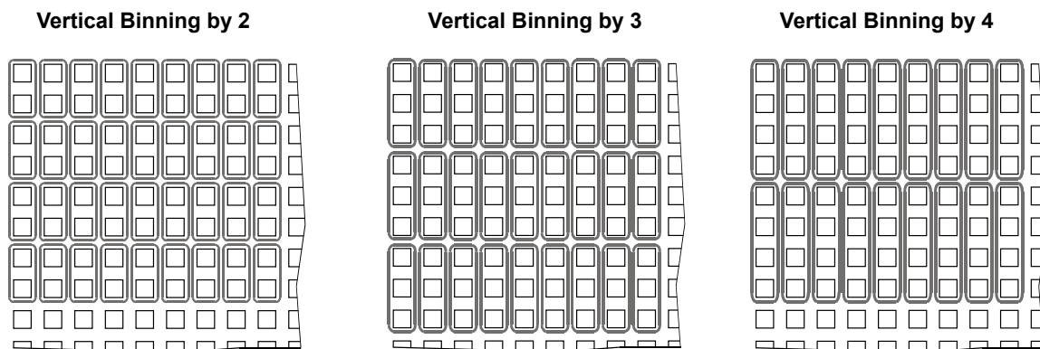
Fig. 63: Vertical Binning
