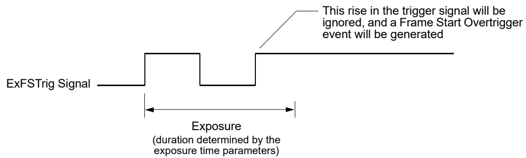
Fig. 33: Overtriggering with Timed Exposure
