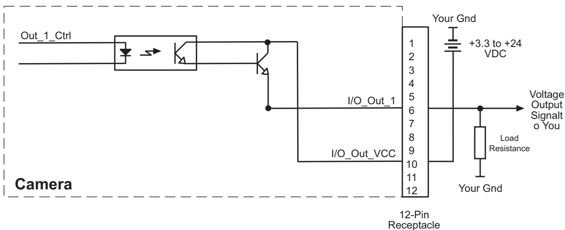
Fig. 24: Typical Voltage Output Circuit
