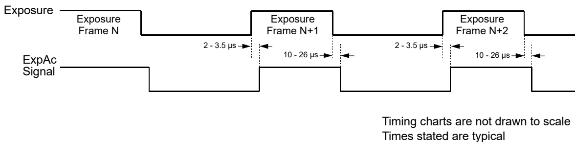
Fig. 46: Exposure Active Signal
