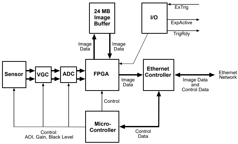
Fig. 19: Camera Block Diagram
