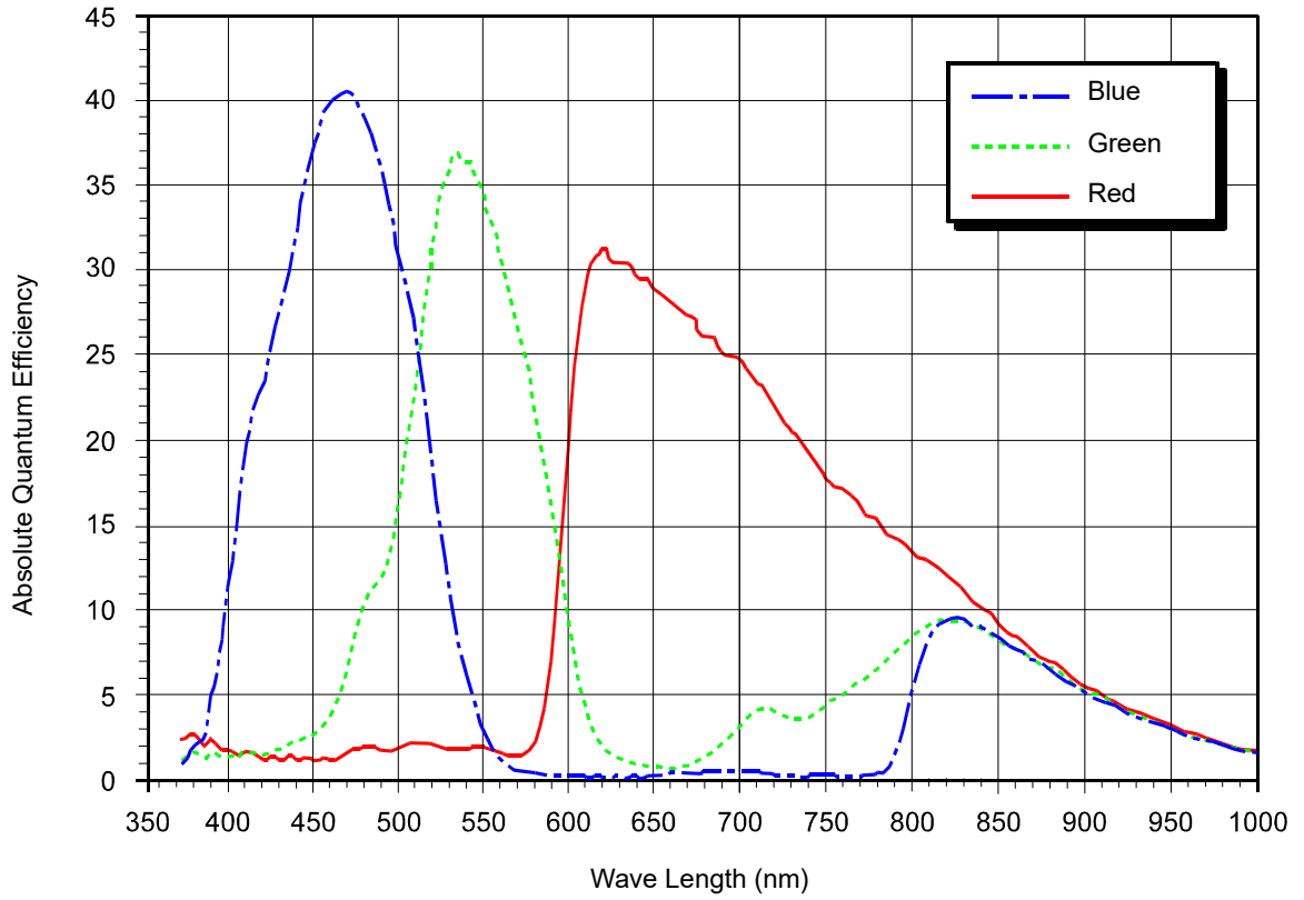
Fig. 6: piA1000-48gc and piA1000-60gc Spectral Response
