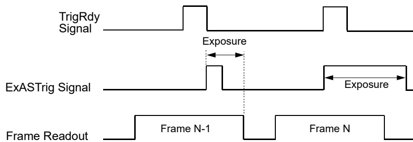
Fig. 39: Trigger Width Exposure Mode with Overlapped Exposure
