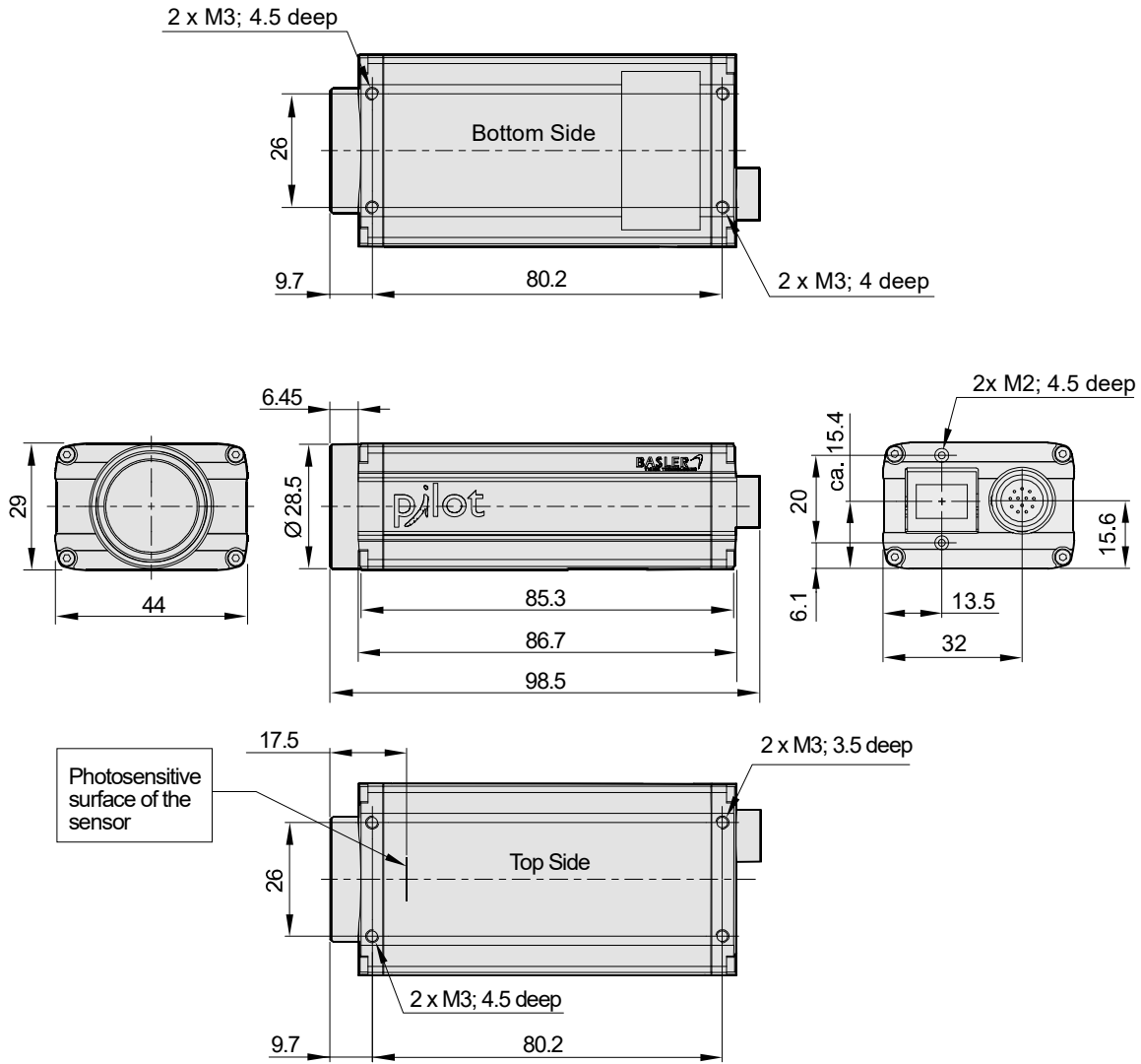
Fig. 9: Mechanical Dimensions (in mm)
