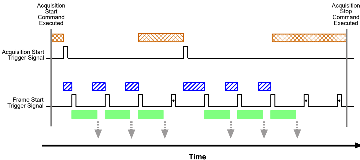
Fig. 30: Acquisition Start and Frame Start Triggering
