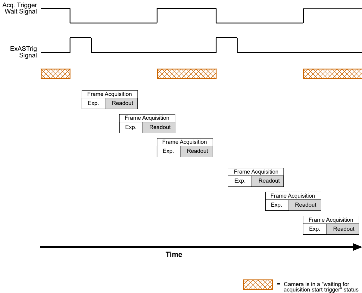
Fig. 48: Acquisition Trigger Wait Signal
