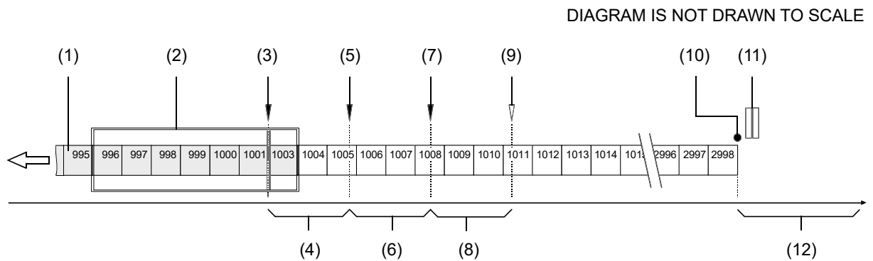
Fig. 16: Combination of Threshold Resend Mechanism and Timeout Resend Mechanism
