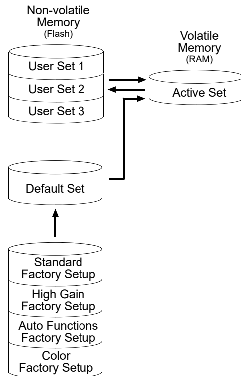
Fig. 77: Configuration Sets
