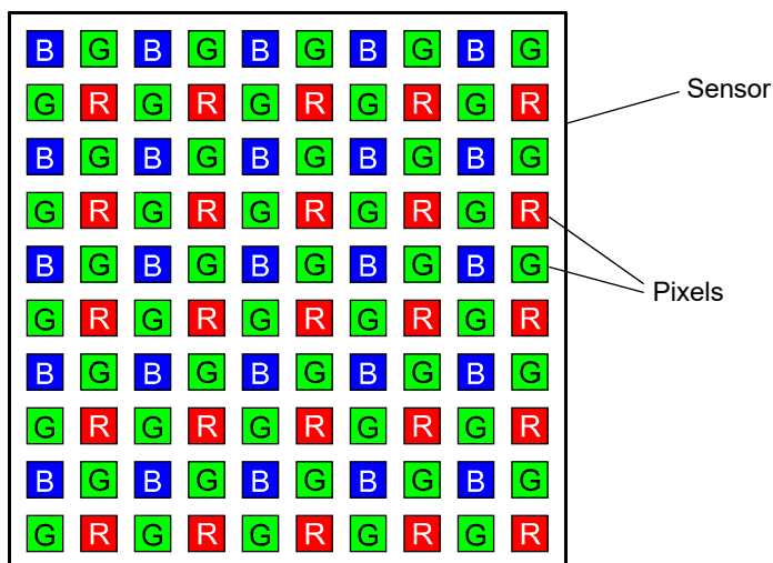
Fig. 50: Bayer Filter Pattern
