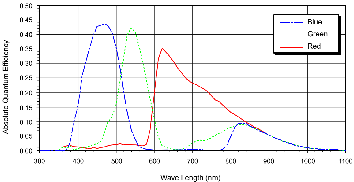
Fig. 5: piA640-210gc Spectral Response
