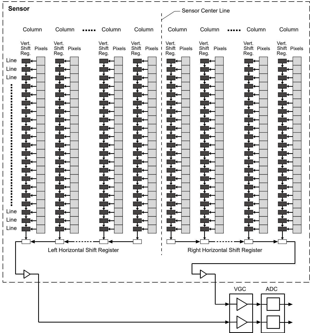
Fig. 18: CCD Sensor Architecture
