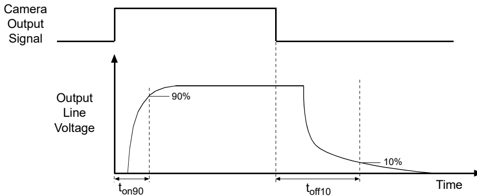
Fig. 25: Output Line Response Times
