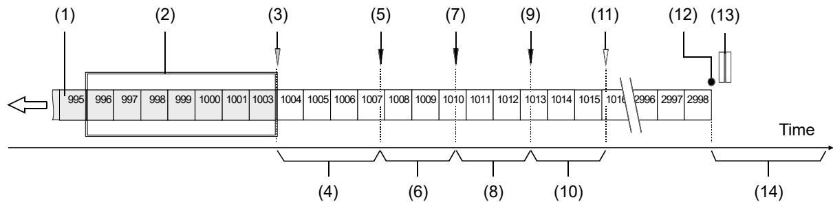
Fig. 15: Incomplete Stream of Packets and Part of the Resend Mechanism
