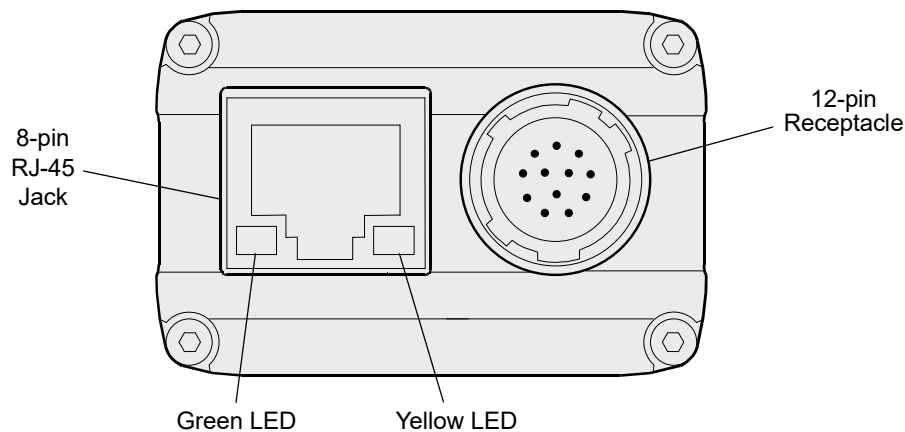
Fig. 20: Camera Connectors and LED
