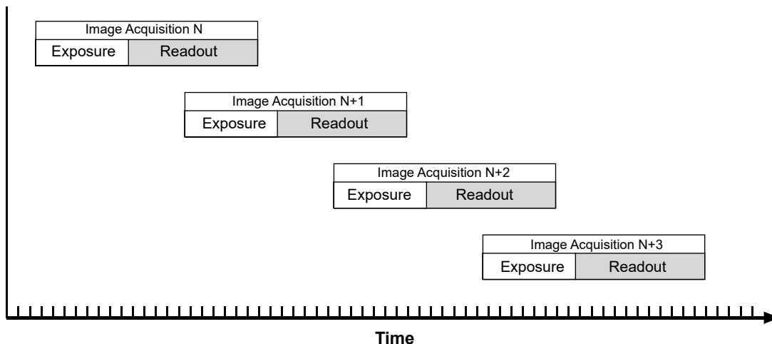
Fig. 45: Overlapped Exposure
