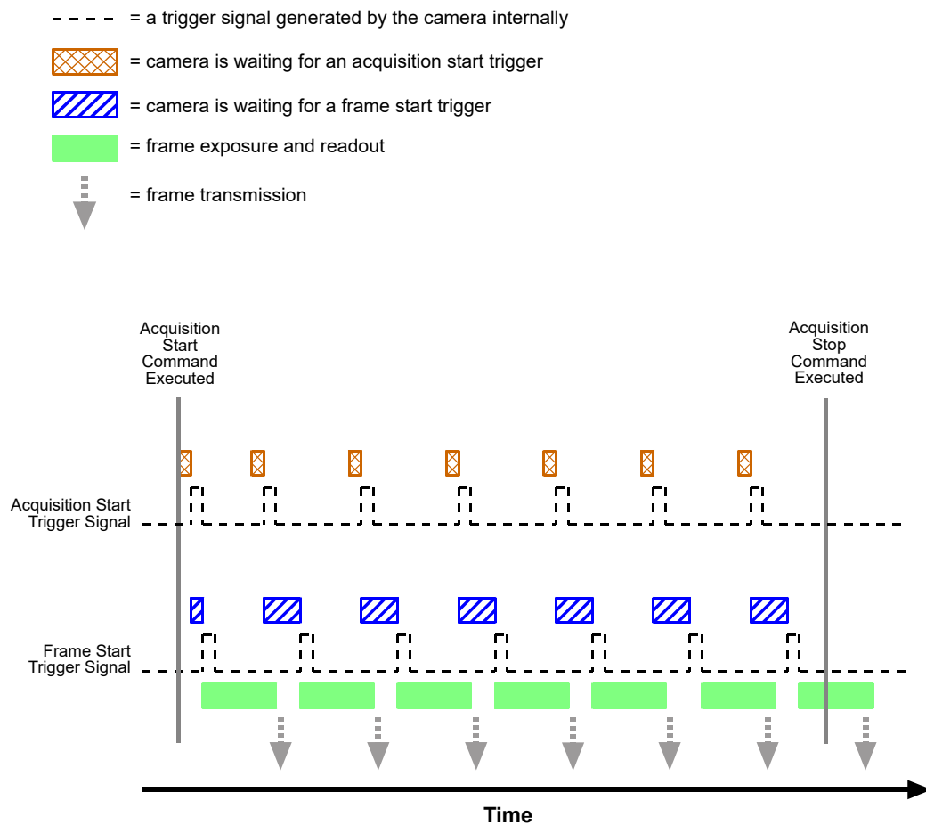
Fig. 40: Use Case 1 - Acquisition Start Trigger Off and Frame Start Trigger Off
