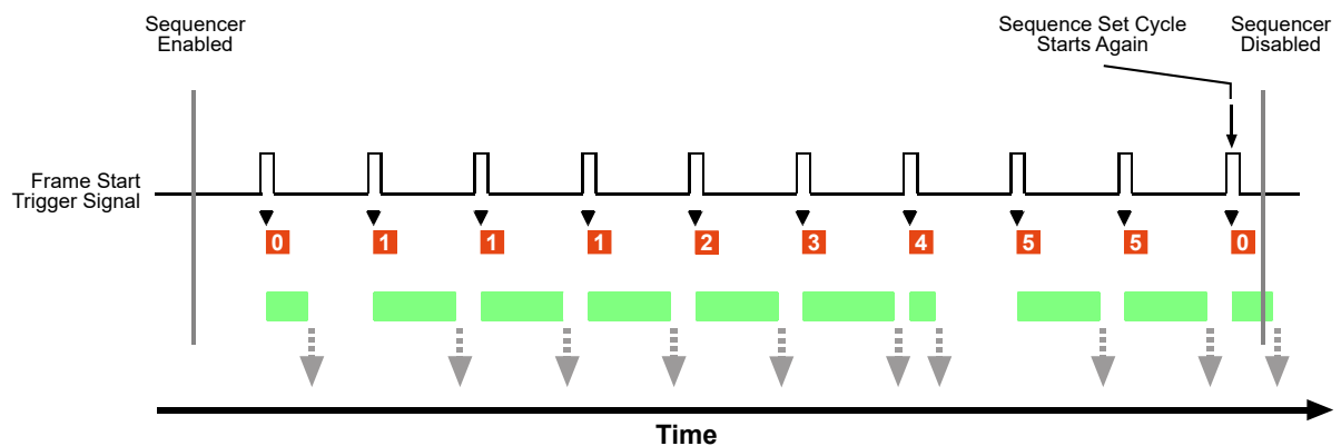
Fig. 56: Sequencer in Auto Sequence Advance Mode
