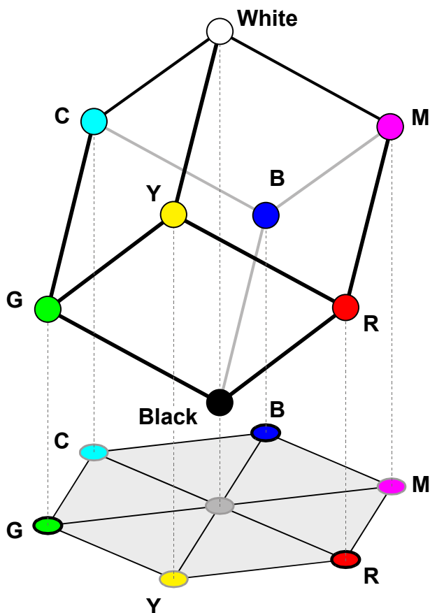
Fig. 51: RGB Color Cube With YCM Secondary Colors, Black, and White, Projected On a Plane
