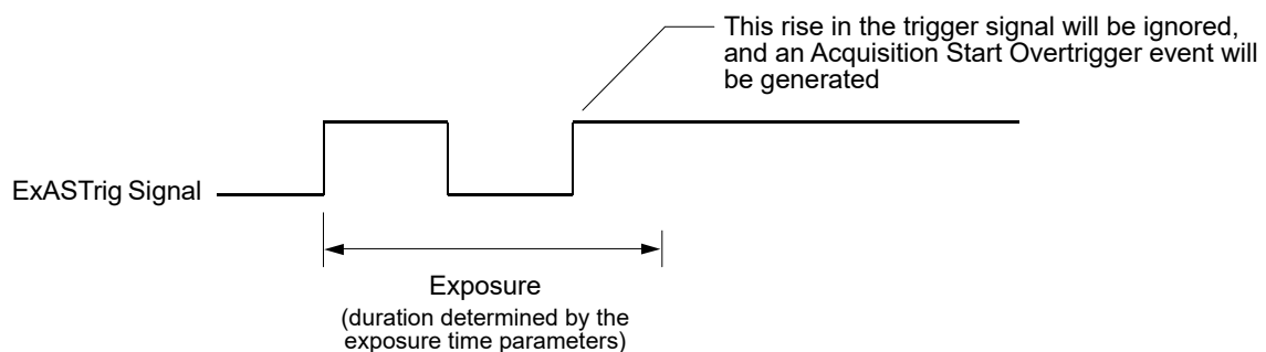
Fig. 37: Overtriggering with Timed Exposure
