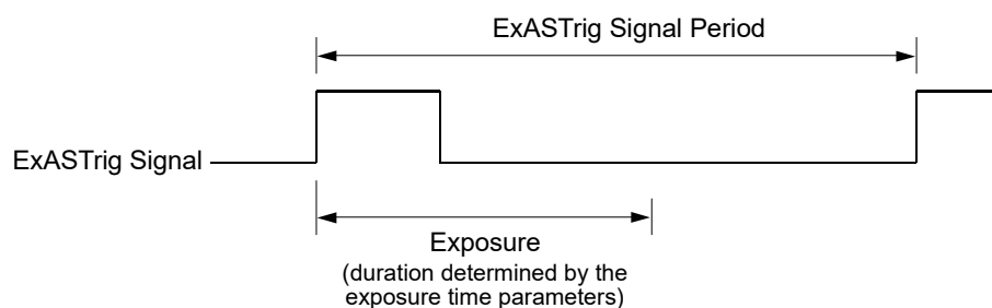
Fig. 36: Timed Exposure with Rising Edge Triggering
