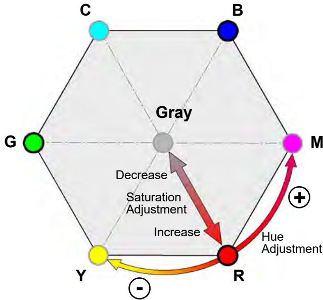
Fig. 52: Hue and Saturation Adjustment In the Color Hexagon. Adjustments Are Indicated for Red as an Example
