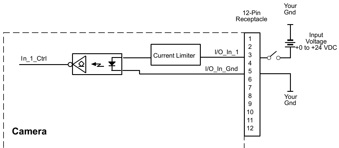
Fig. 23: Typical Voltage Input Circuit
