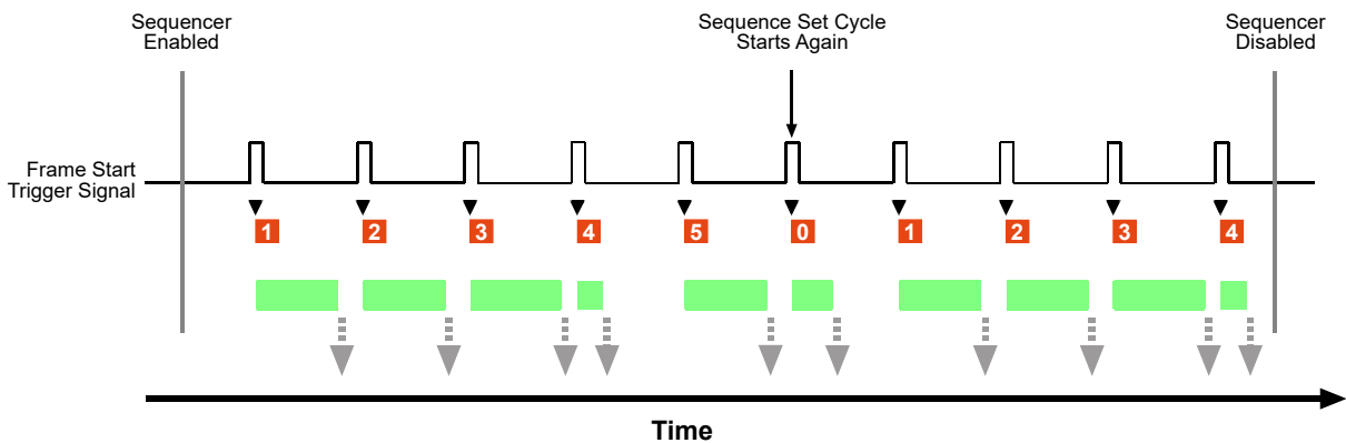
Fig. 57: Sequencer in Controlled Sequence Advance Mode with Always Active as the Sequence Control Source
