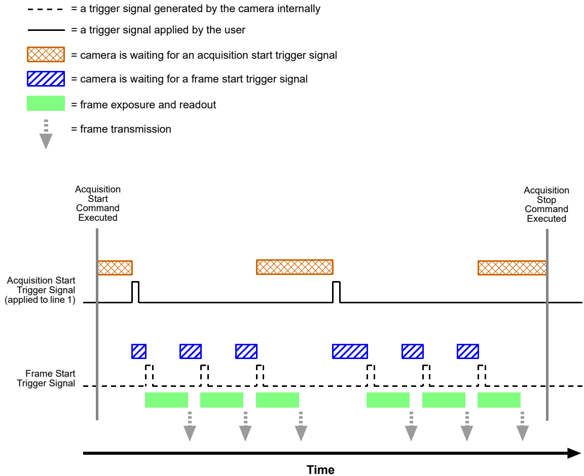
Fig. 42: Use Case 3 - Acquisition Start Trigger On and Frame Start Trigger Off
