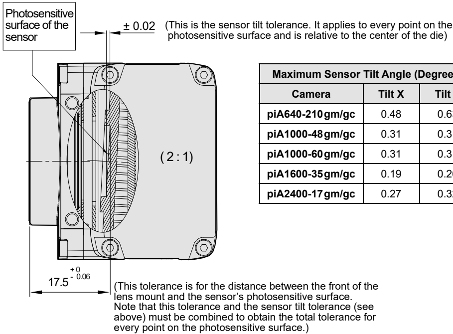
Fig. 12: Sensor Positioning Accuracy for Cameras With 90° Head Housing (in mm unless otherwise noted)
