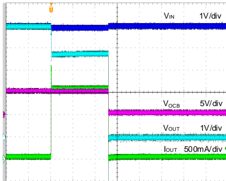
SY20807L Over Current Response
