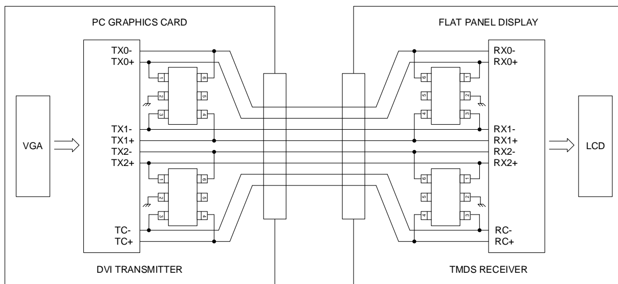
Layout Top View for Digital Visual Interface (DVI) with SY205236ABC
