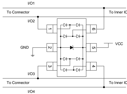
Figure 1. SY205214ABC Pin Connections in PCB
