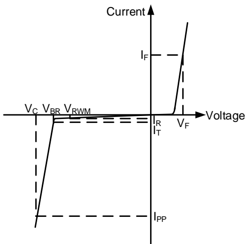
Figure 1. Uni-directional TVS
