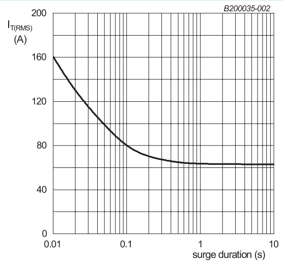
Fig. 2. RMS on-state current as a function of surge duration; maximum values f = 50\text{ Hz} ; T_{mb} = 106\text{ °C}
