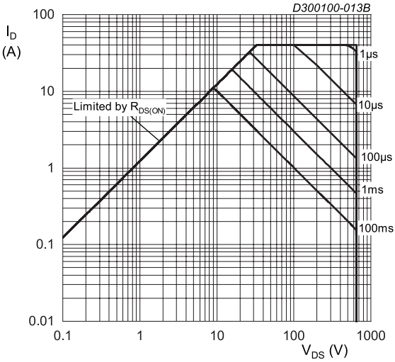
Fig. 13. Safe operating area T_{mb} = 25\text{ }^{\circ}\text{C}
