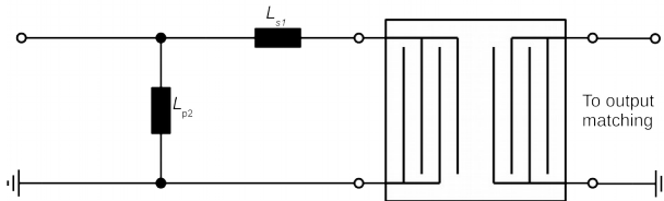
Figure 14: shunt L - series L matching.
