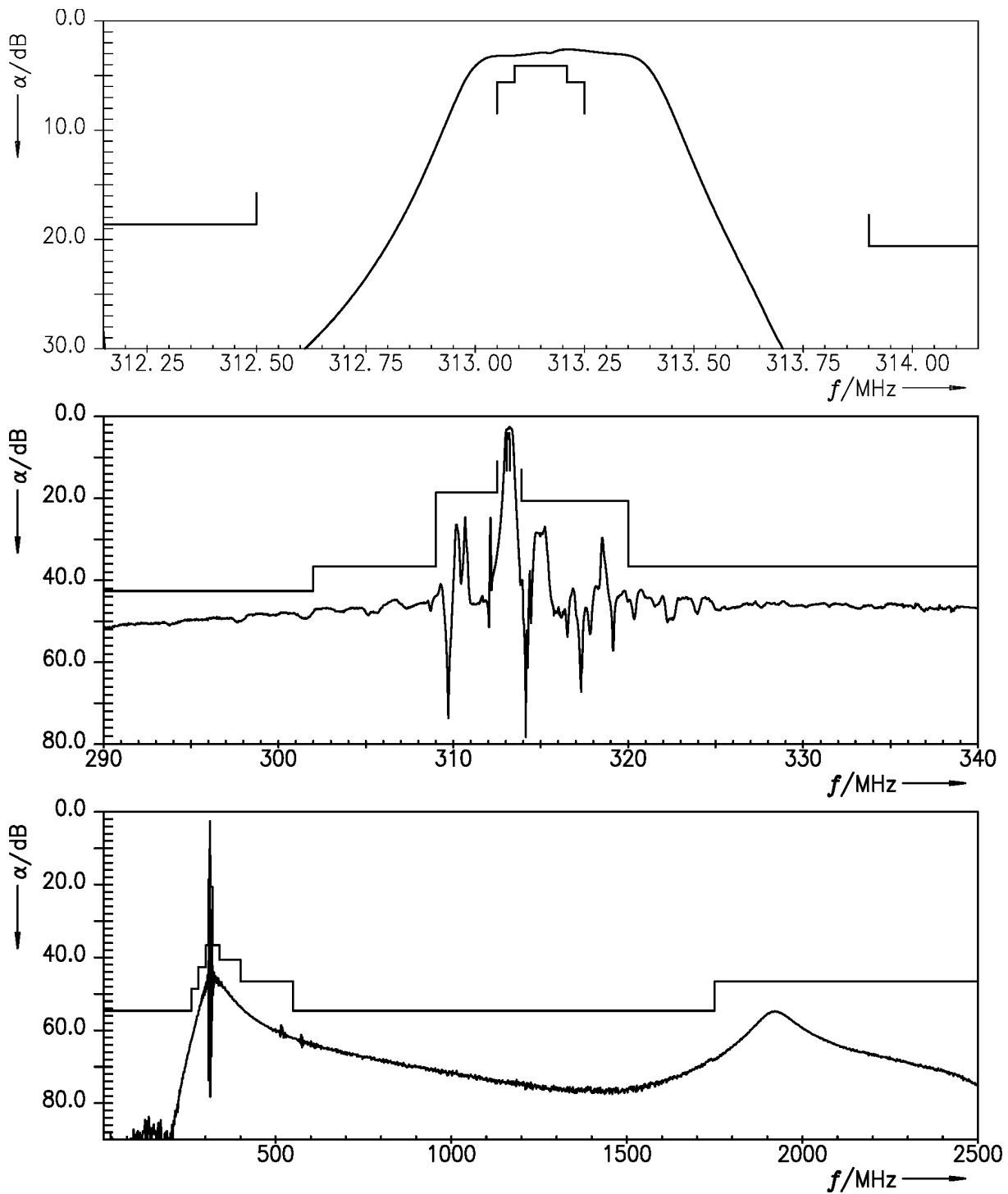
Figure 6: Attenuation Channel 2.
