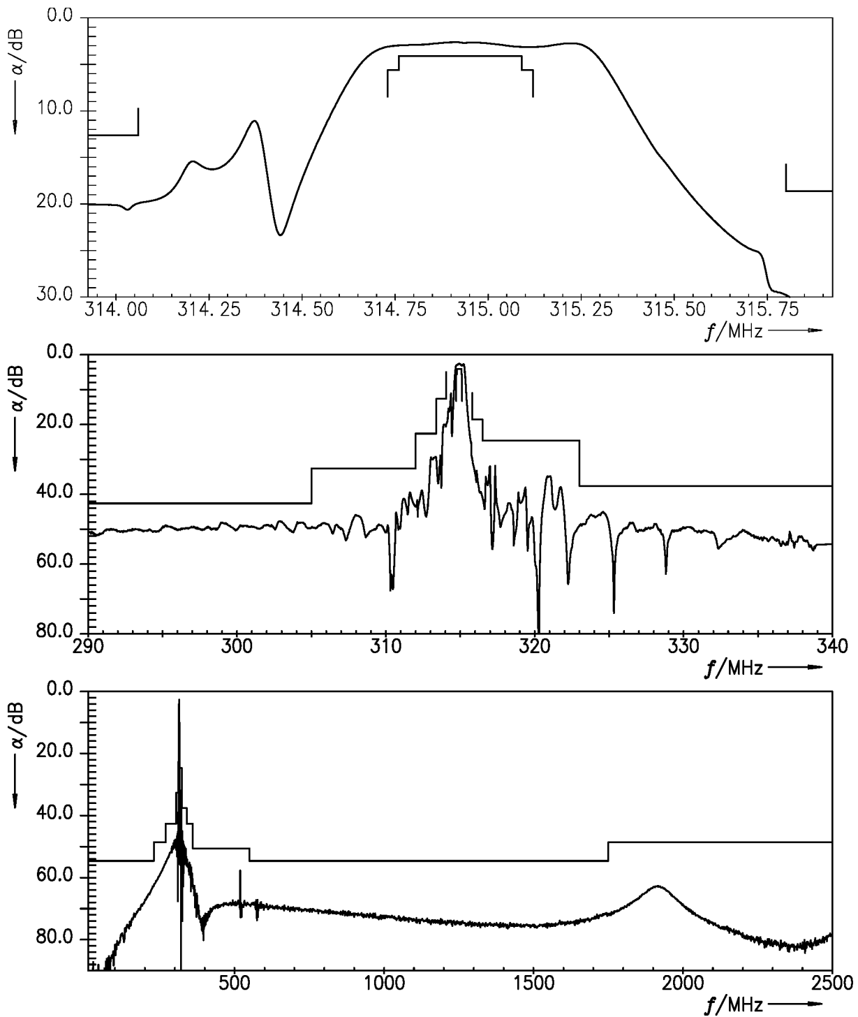
Figure 5: Attenuation Channel 1.
