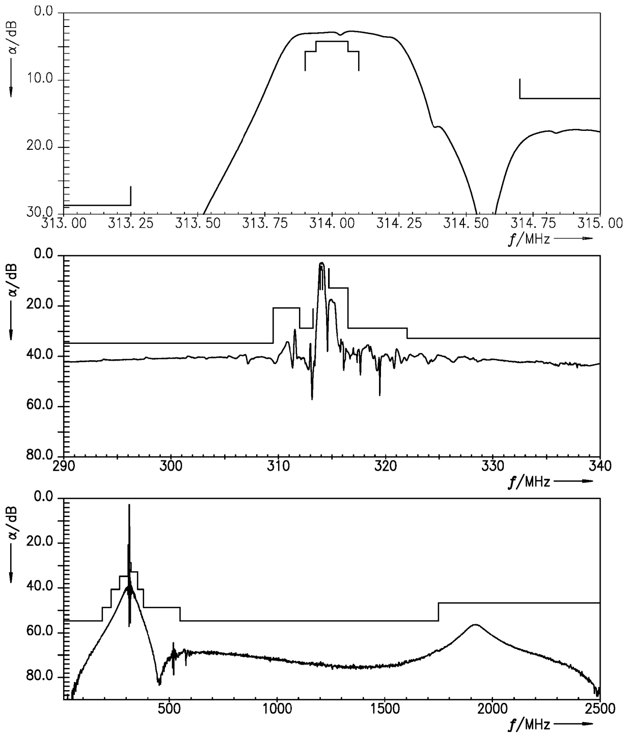
Figure 7: Attenuation Channel 3.
