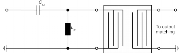
Figure 15: series C - shunt L matching.
