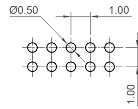
Recommended PCB Layout General TOL: ±0.05
