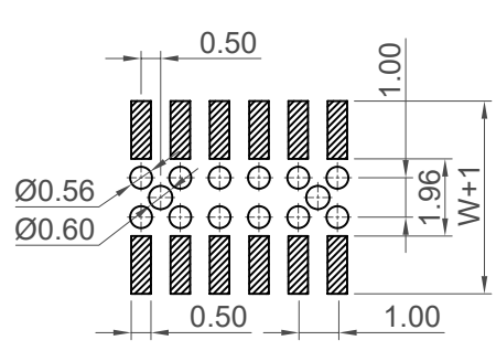
Recommended PCB Layout For Bottom Entry General Tolerance: ±0.05 Solder Area
