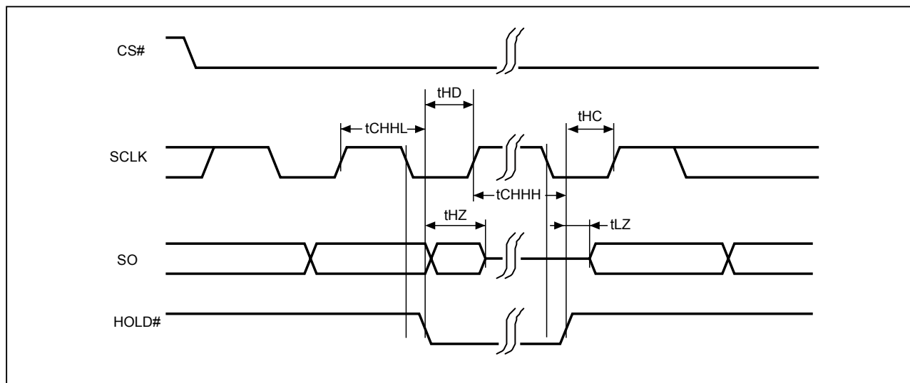
Figure 40. Hold Timing
