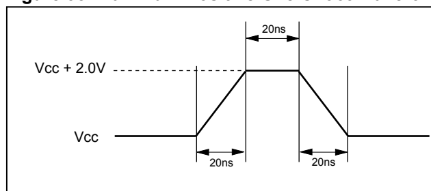
Figure 35. Maximum Positive Overshoot Waveform
