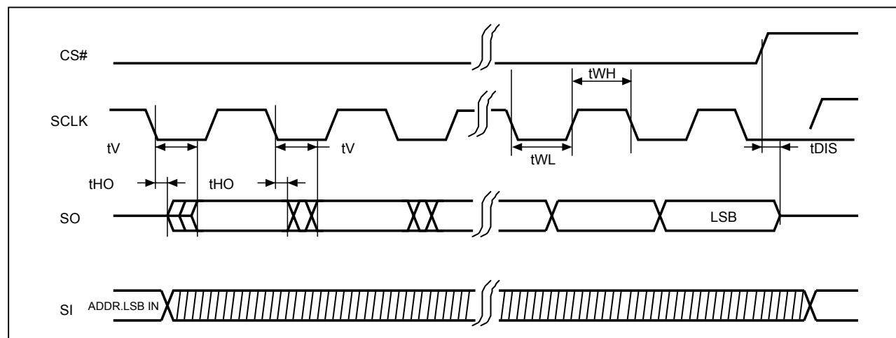
Figure 39. Serial Output Timing
