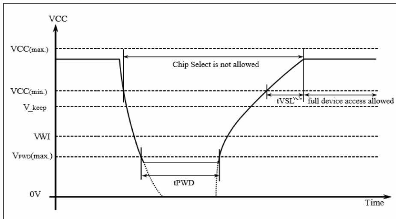
Figure 33. Power Up/Down and Voltage Drop
