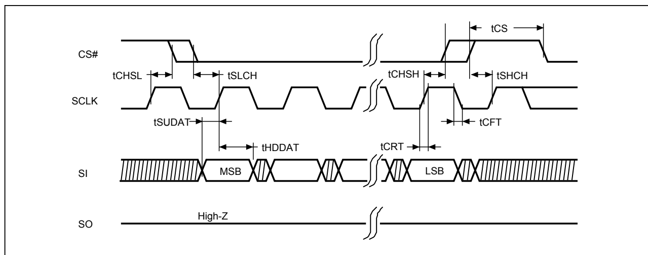
Figure 38. Serial Input Timing
