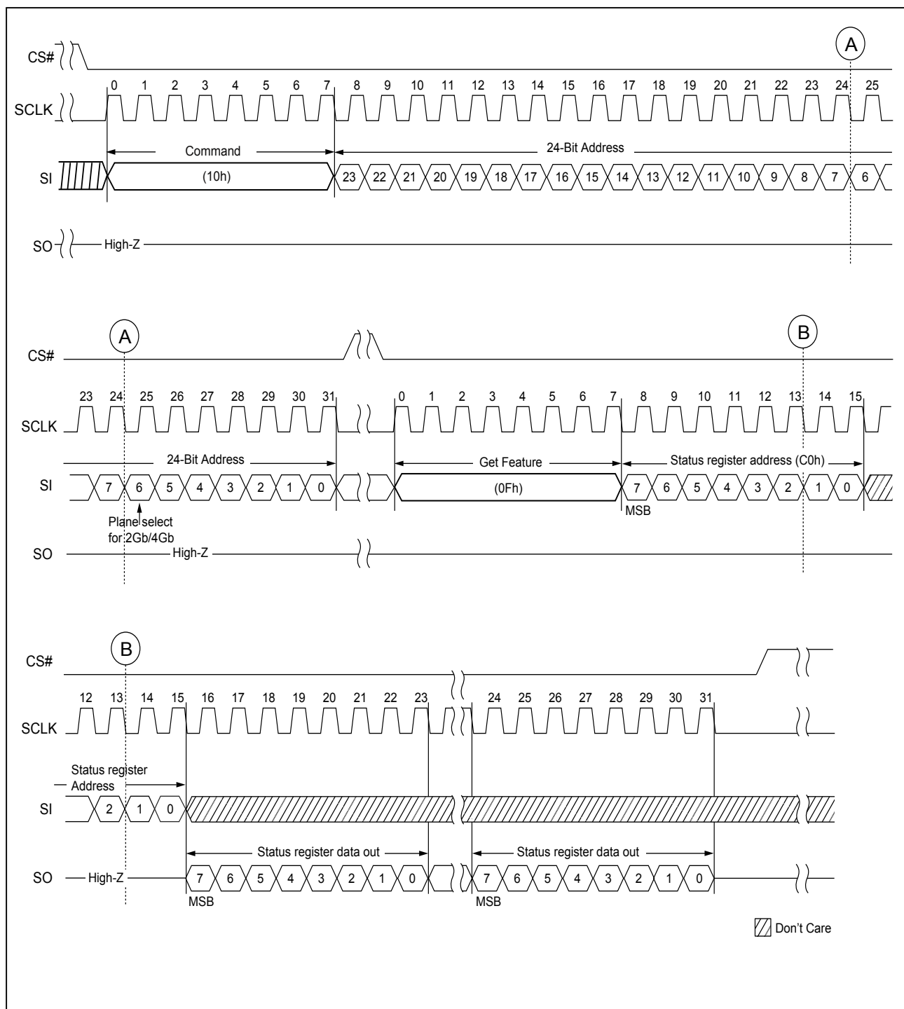
Figure 26. PROGRAM EXECUTE (10h) Timing
