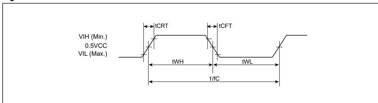
Figure 36. SCLK TIMING DEFINITION
