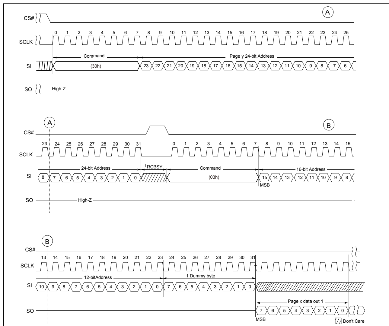
Figure 15. Page Read Cache Random (30h)
