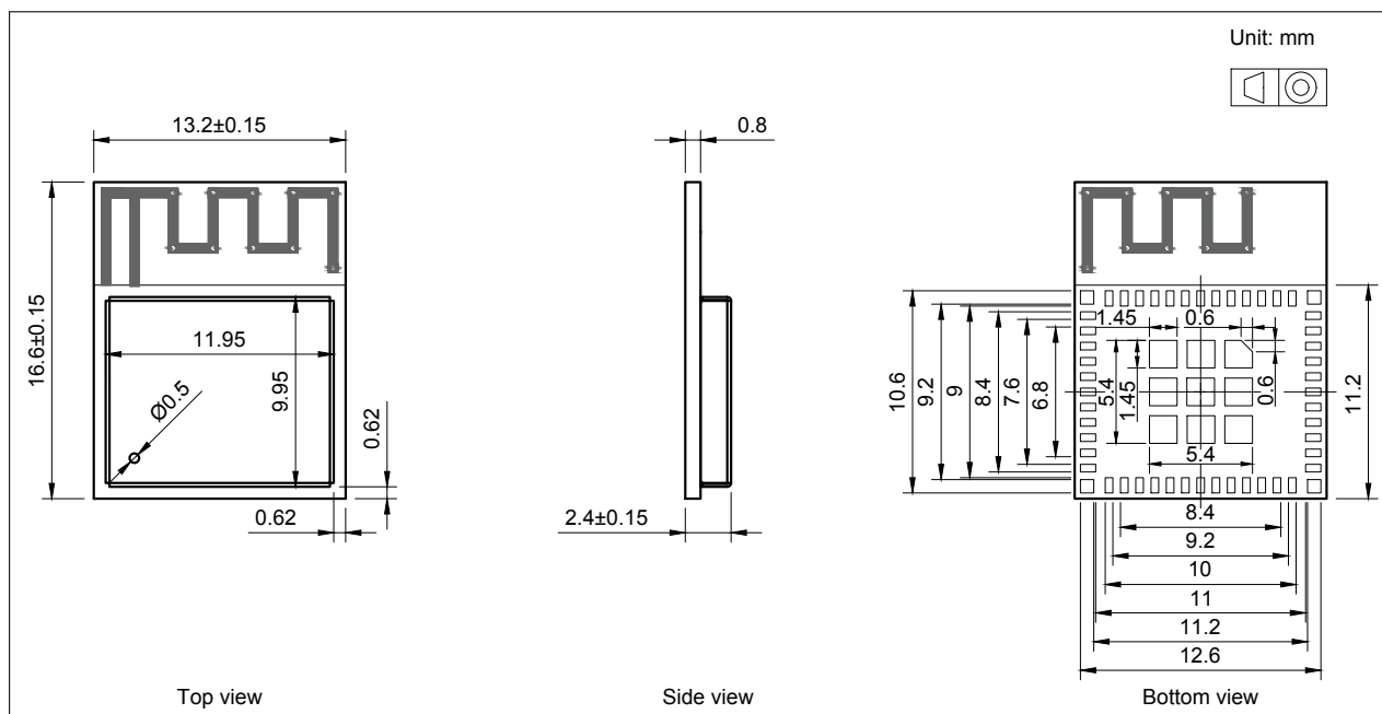
Figure 9: ESP32-PICO-MINI-02 Physical Dimensions
