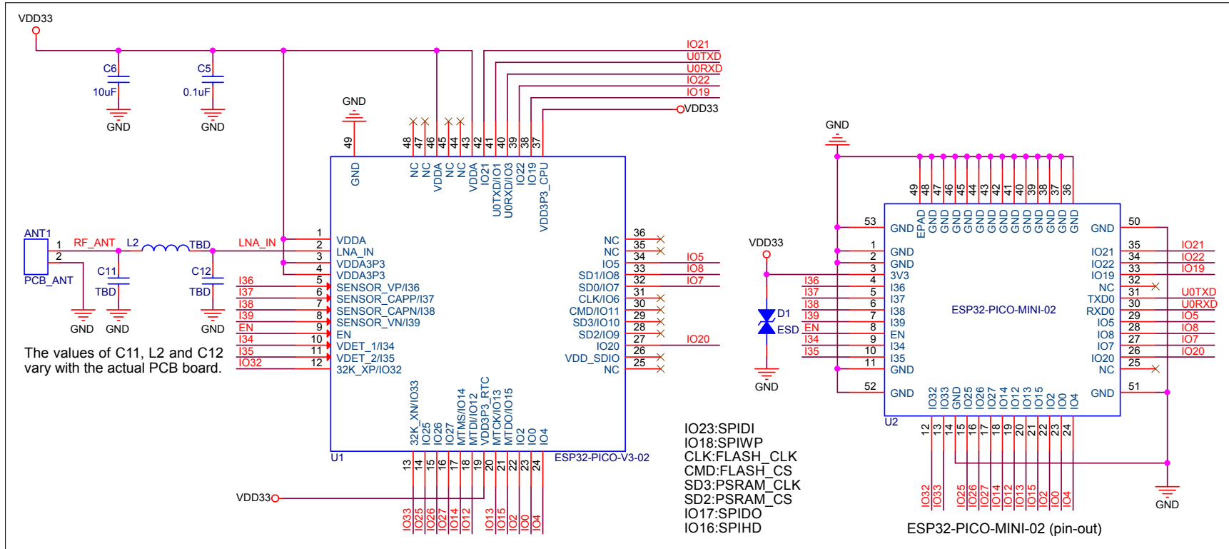
Figure 6: ESP32-PICO-MINI-02 Schematics
